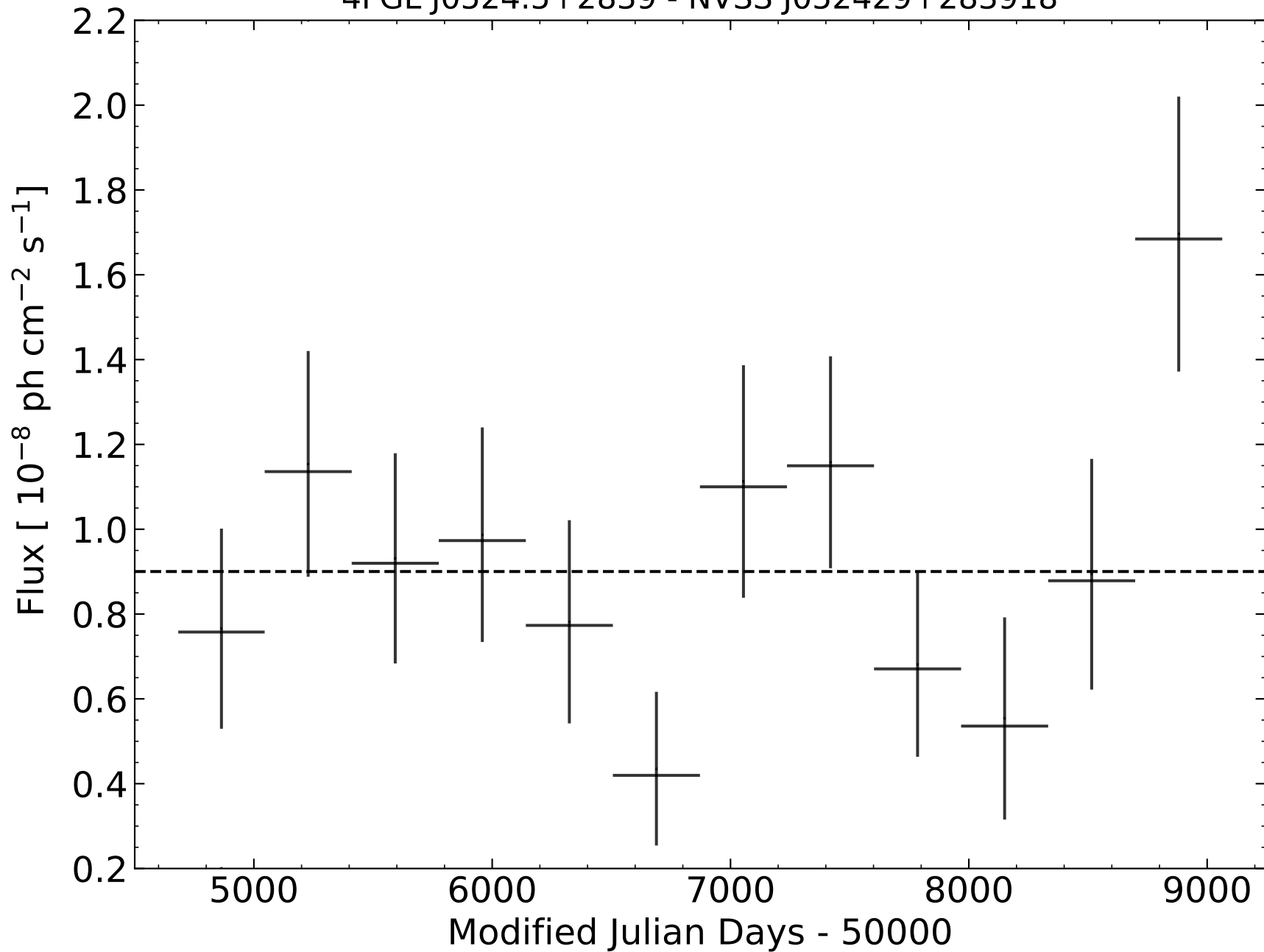
4FGL J0524.5+2839 - NVSS J052429+283918
