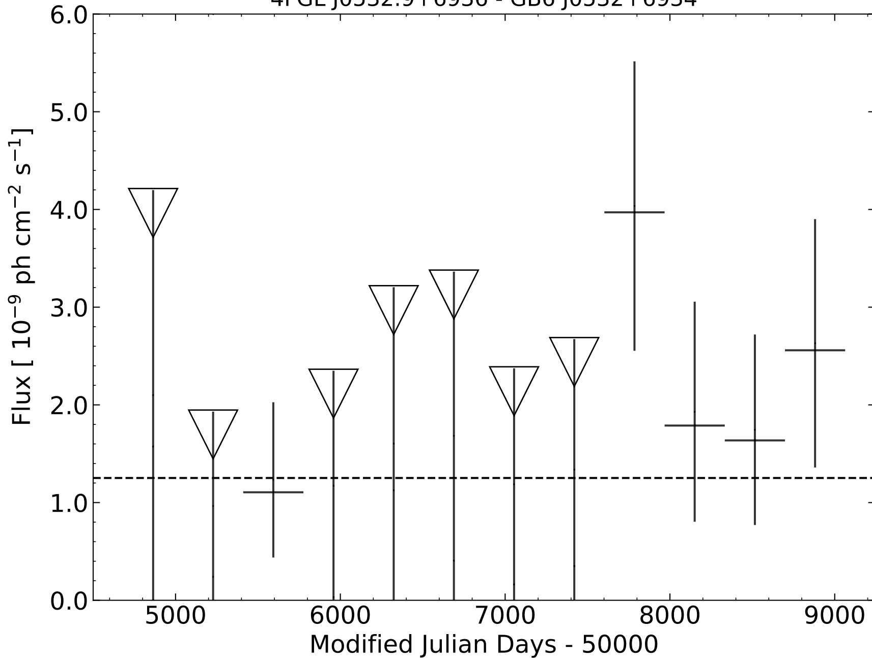
4FGL J0532.9+6936 - GB6 J0532+6934
