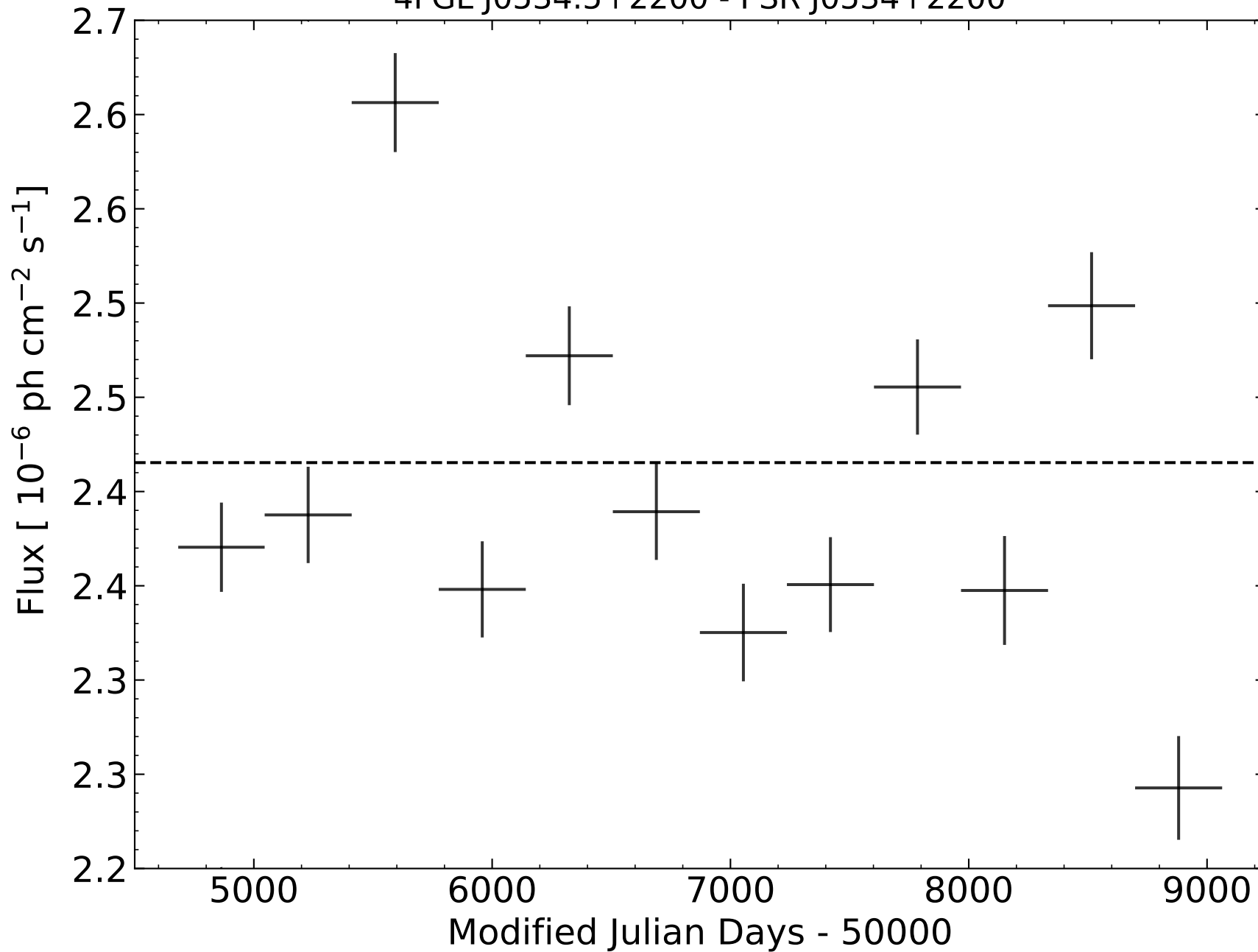
4FGL J0534.5+2200 - PSR J0534+2200
