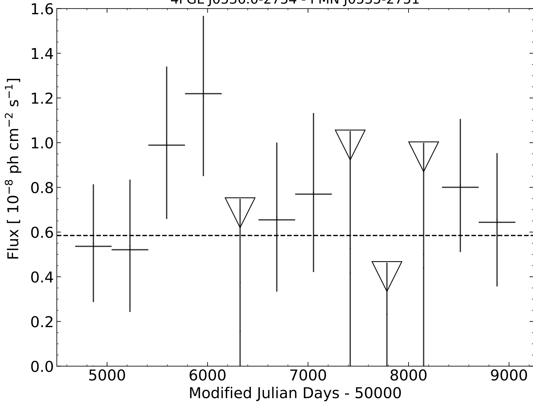
4FGL J0536.0-2754 - PMN J0535-2751
