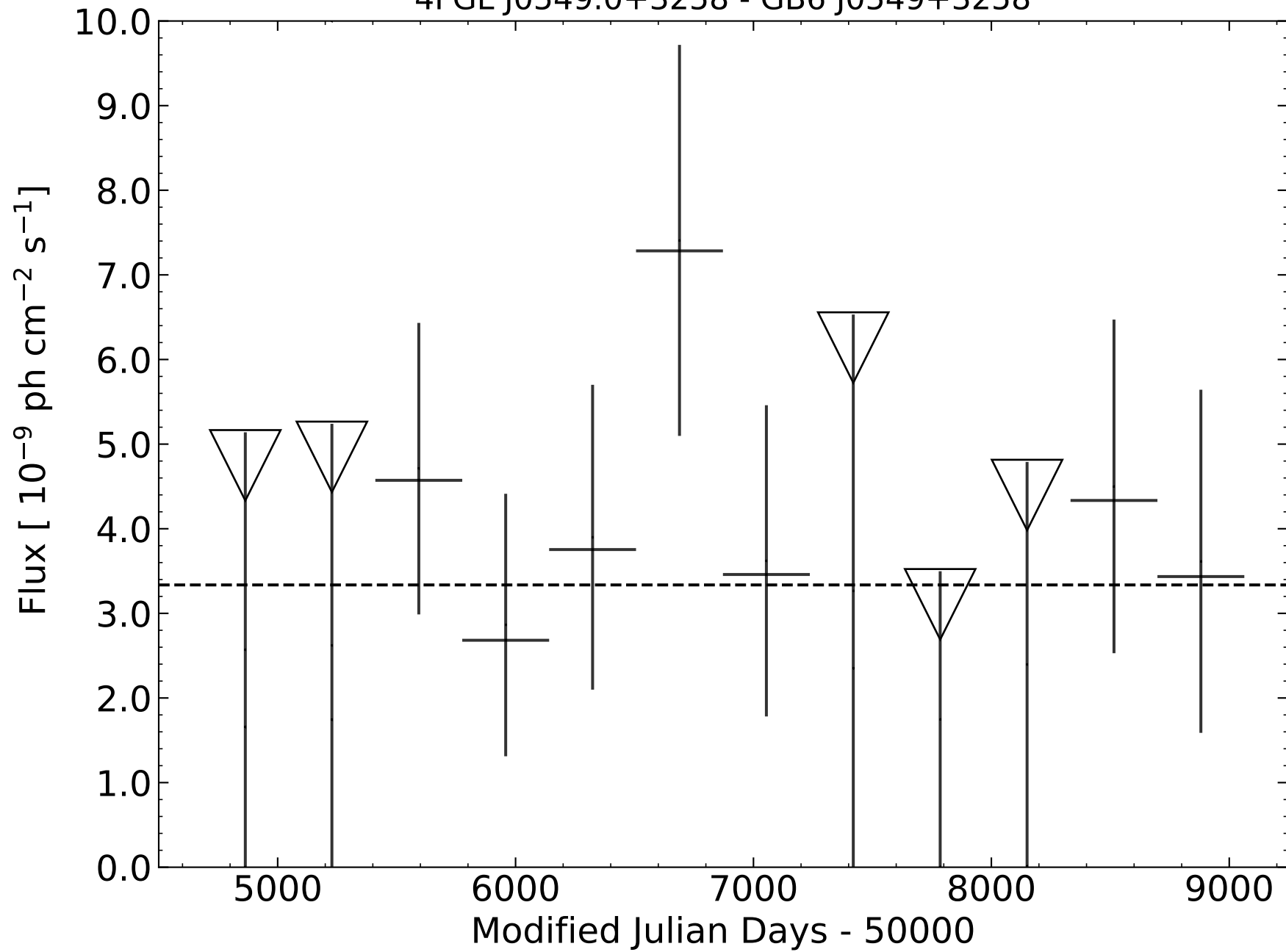
4FGL J0549.0+3258 - GB6 J0549+3258
