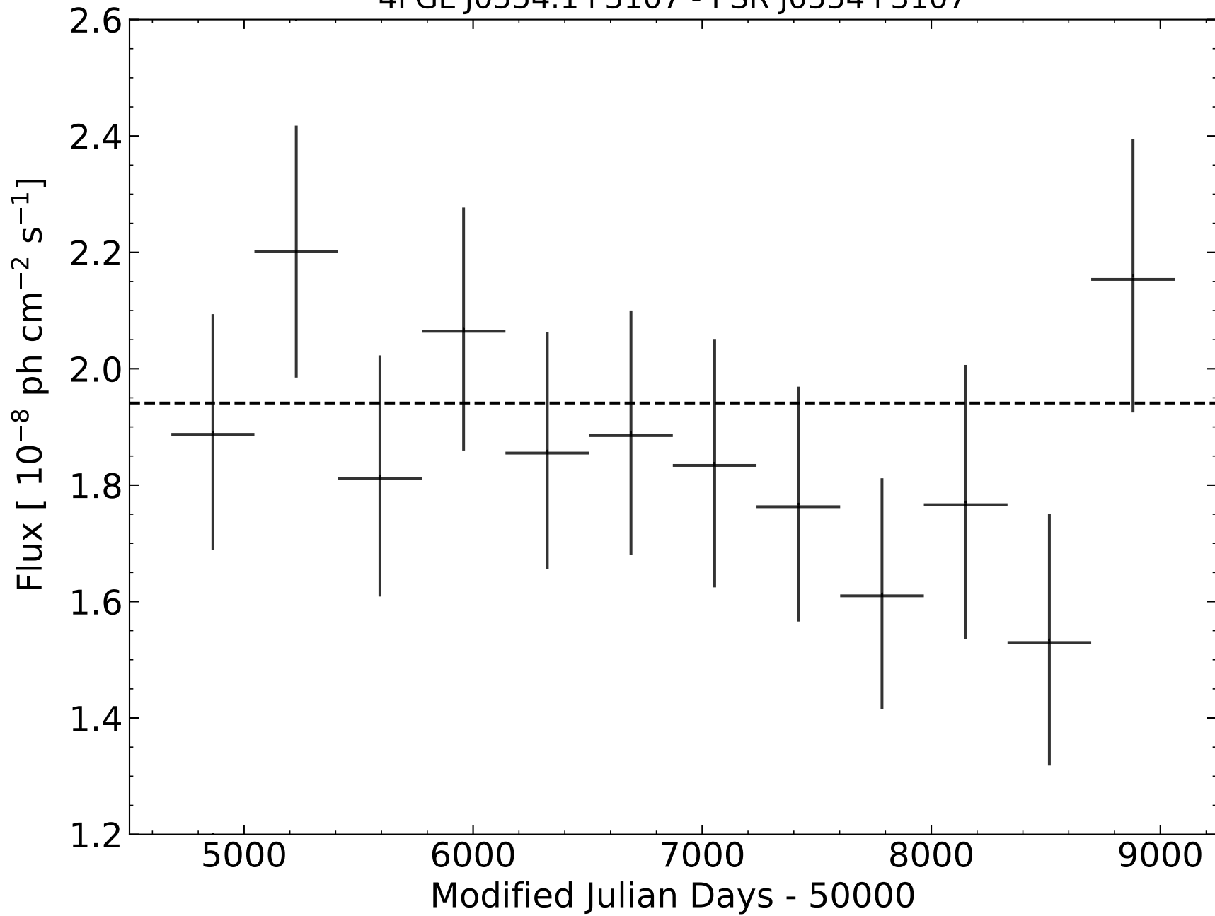
4FGL J0554.1+3107 - PSR J0554+3107
