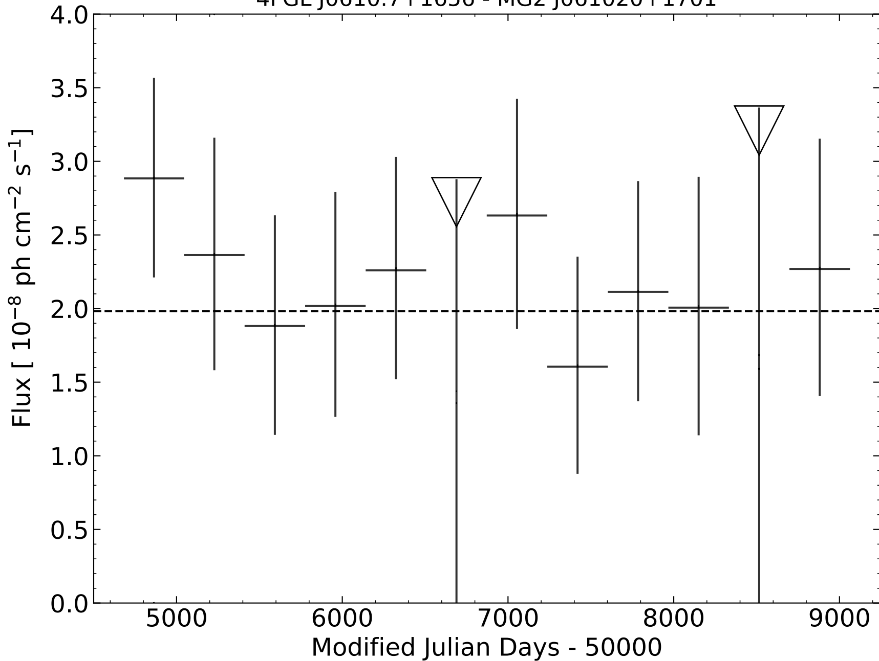
4FGL J0610.7+1656 - MG2 J061020+1701
