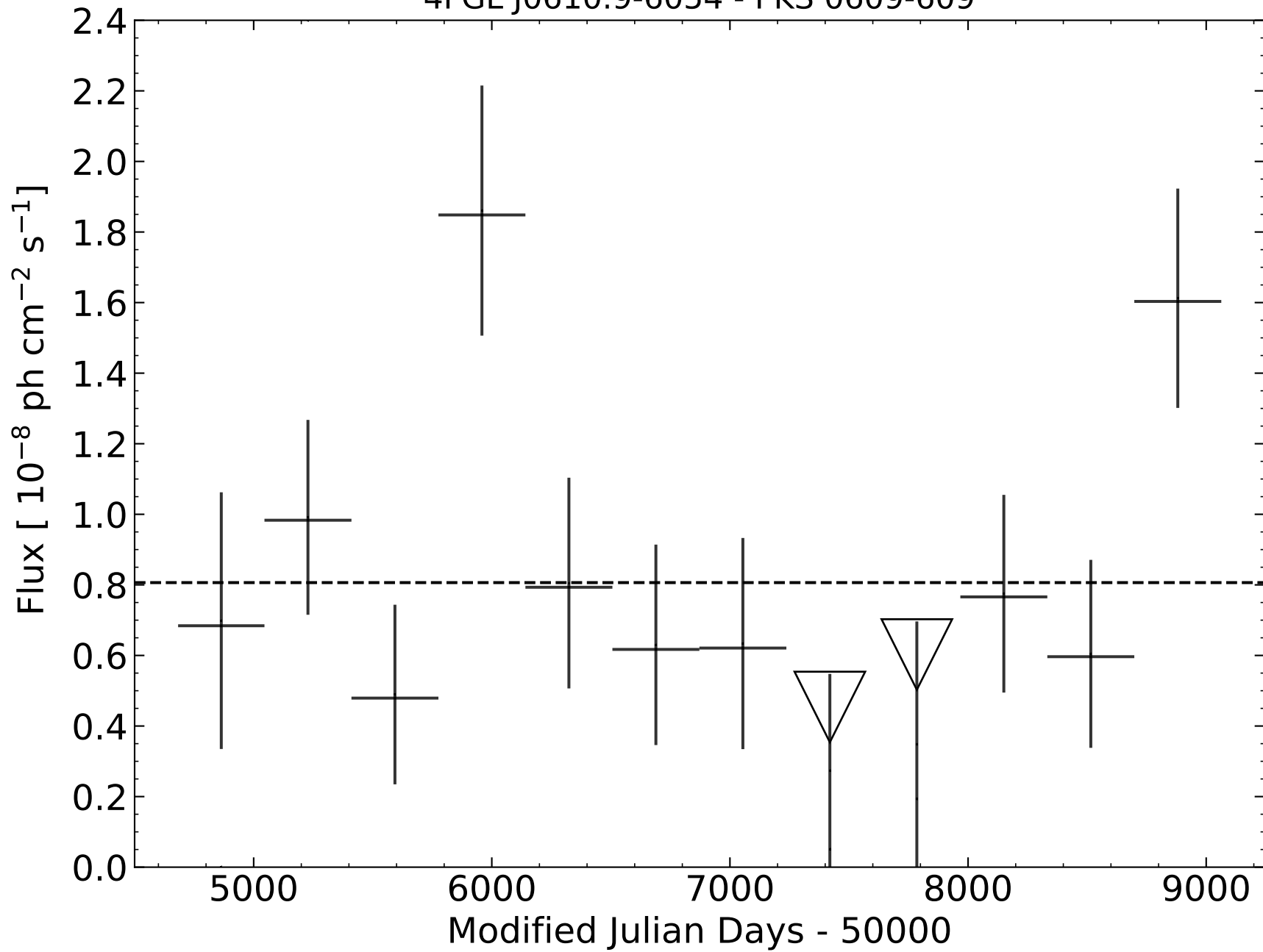
4FGL J0610.9-6054 - PKS 0609-609
