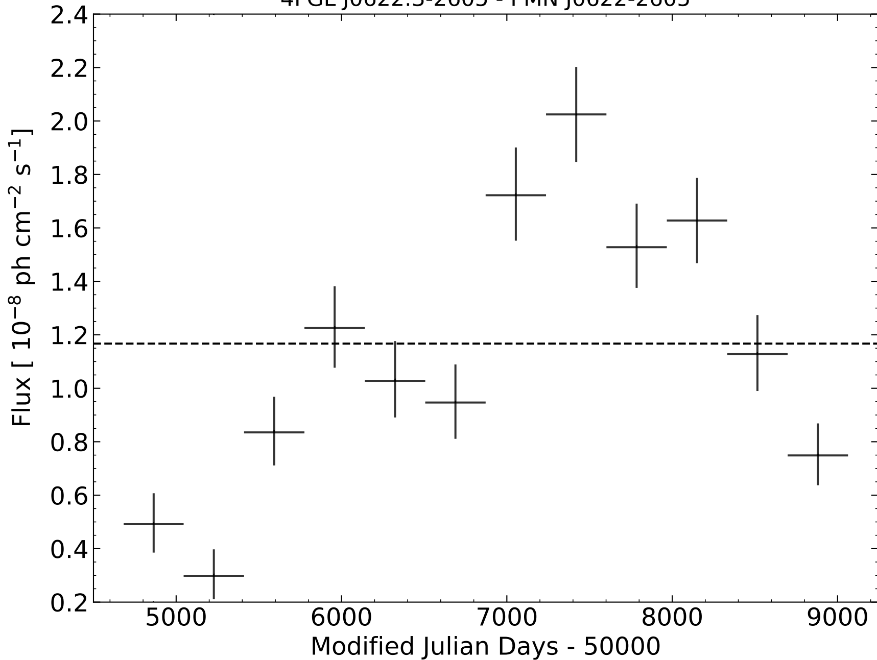
4FGL J0622.3-2605 - PMN J0622-2605
