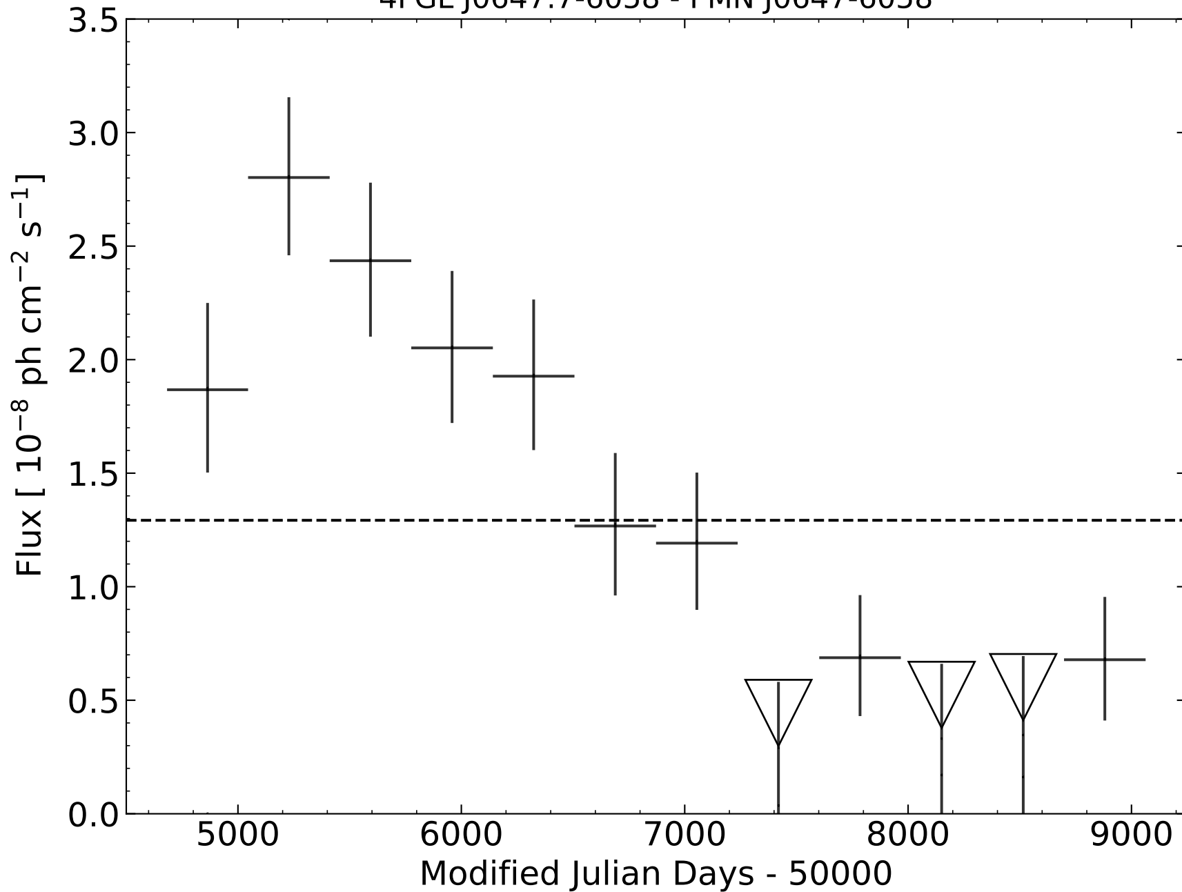
4FGL J0647.7-6058 - PMN J0647-6058
