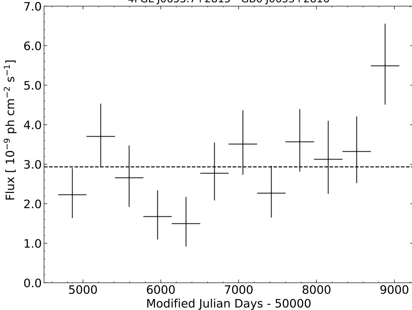
4FGL J0653.7+2815 - GB6 J0653+2816
