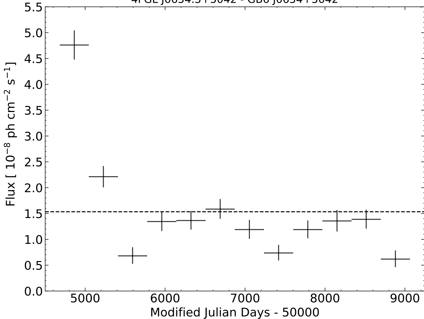
4FGL J0654.3+5042 - GB6 J0654+5042
