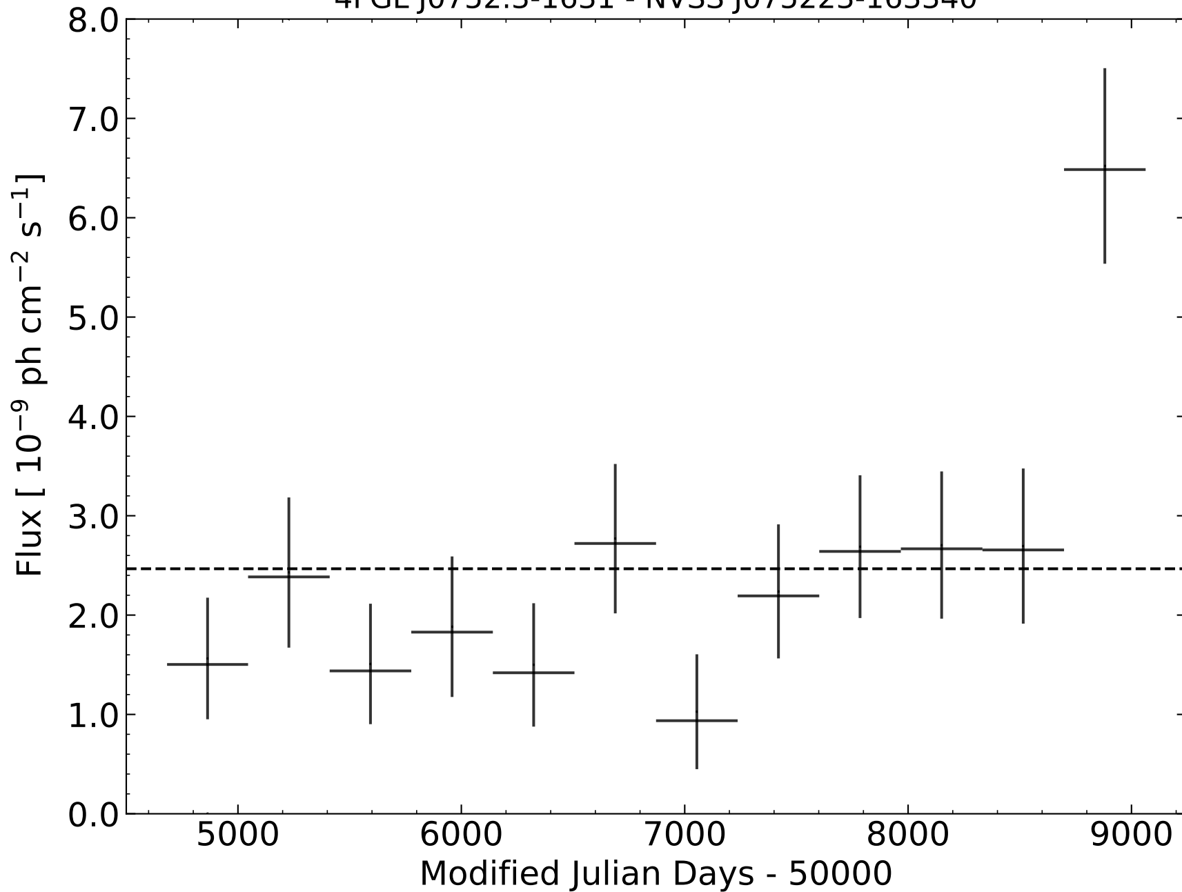
4FGL J0752.3-1631 - NVSS J075223-163340
