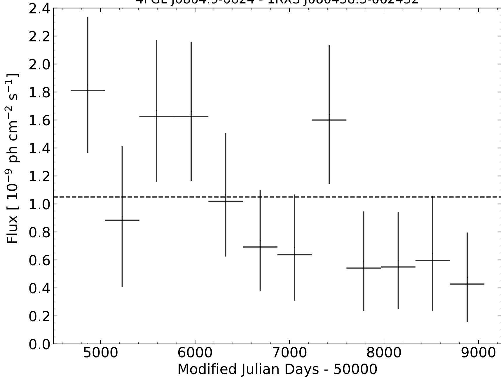
4FGL J0804.9-0624 - 1RXS J080458.3-062432
