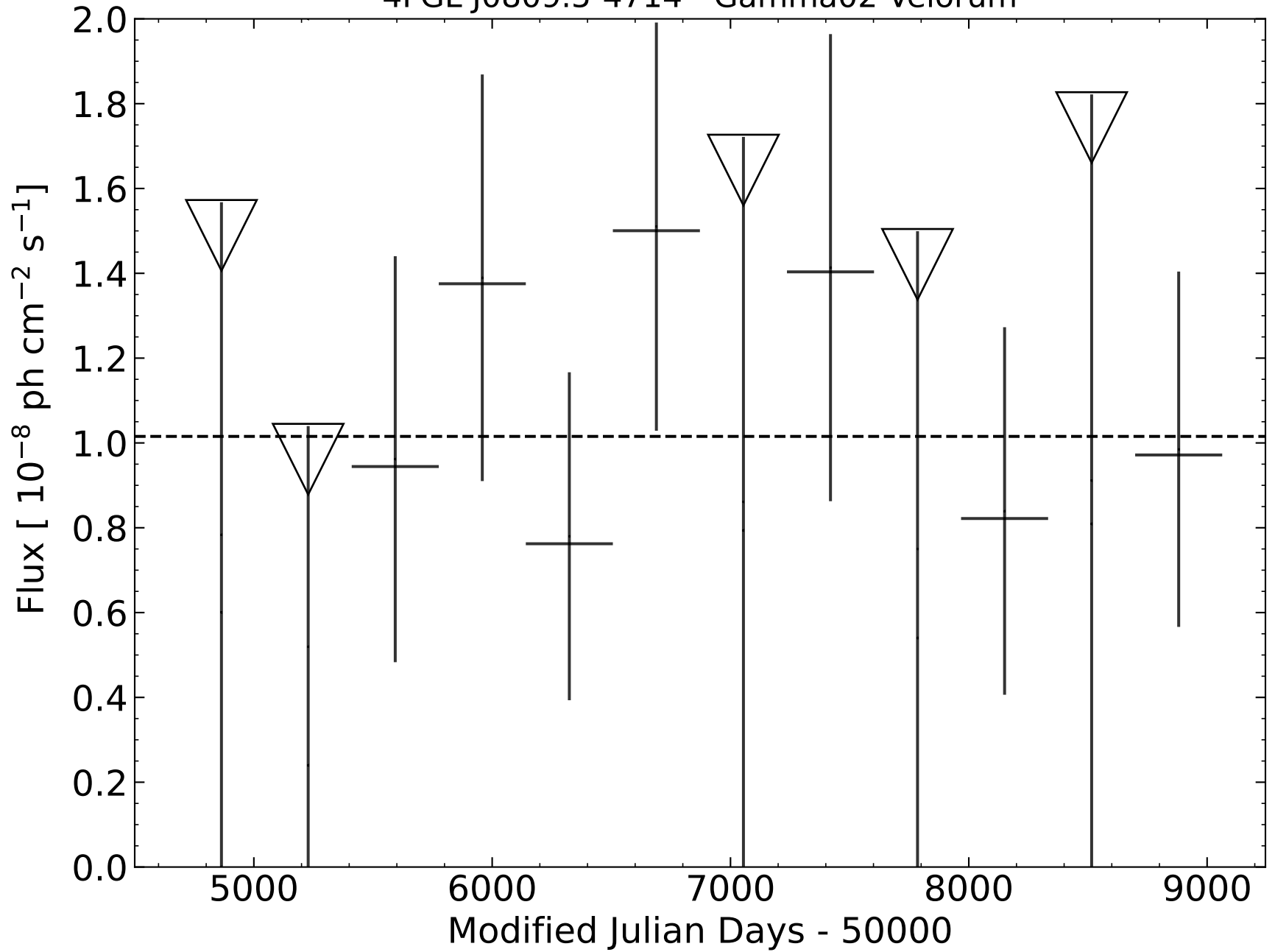
4FGL J0809.5-4714 - Gamma02 Velorum
