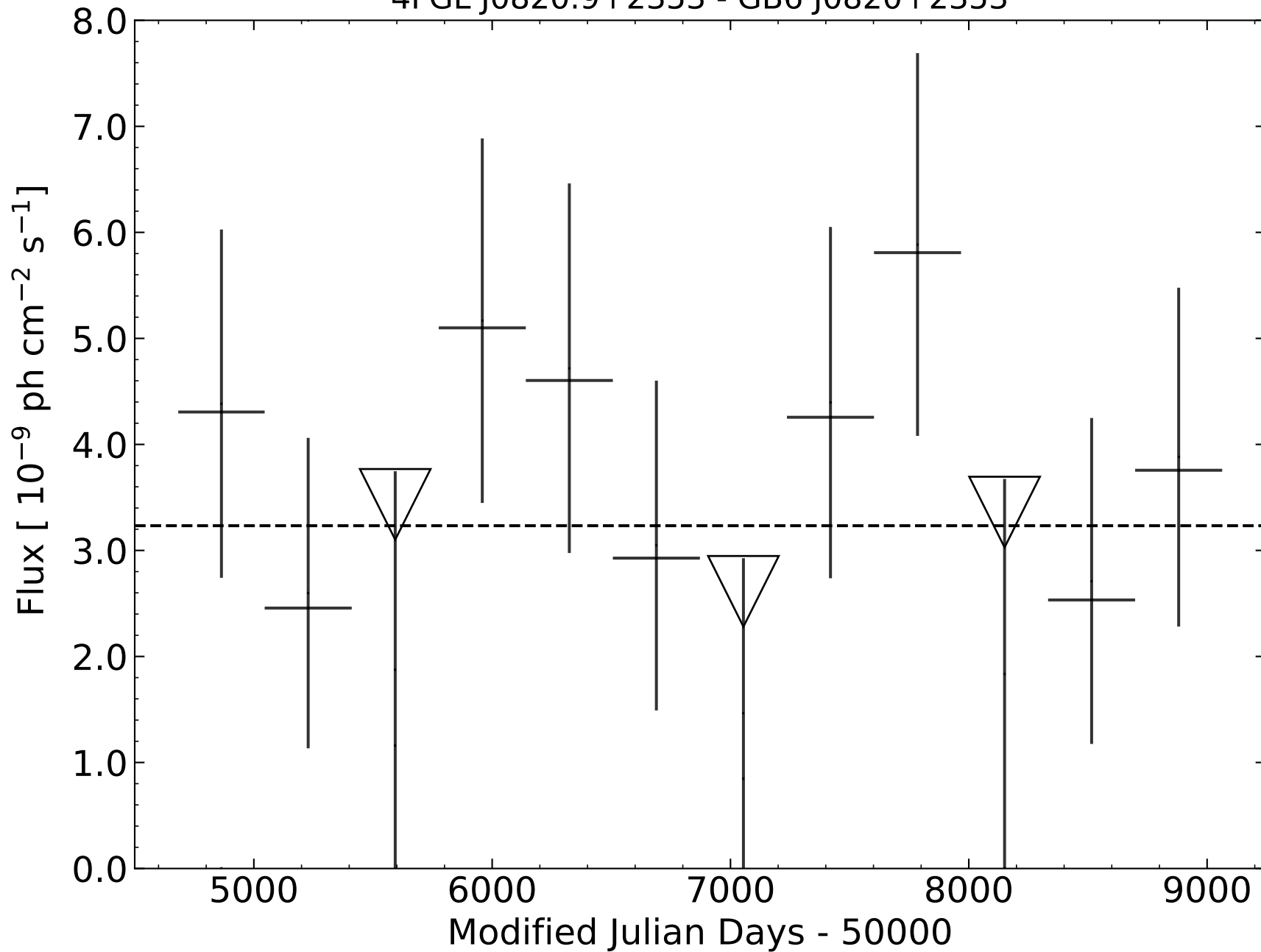
4FGL J0820.9+2353 - GB6 J0820+2353
