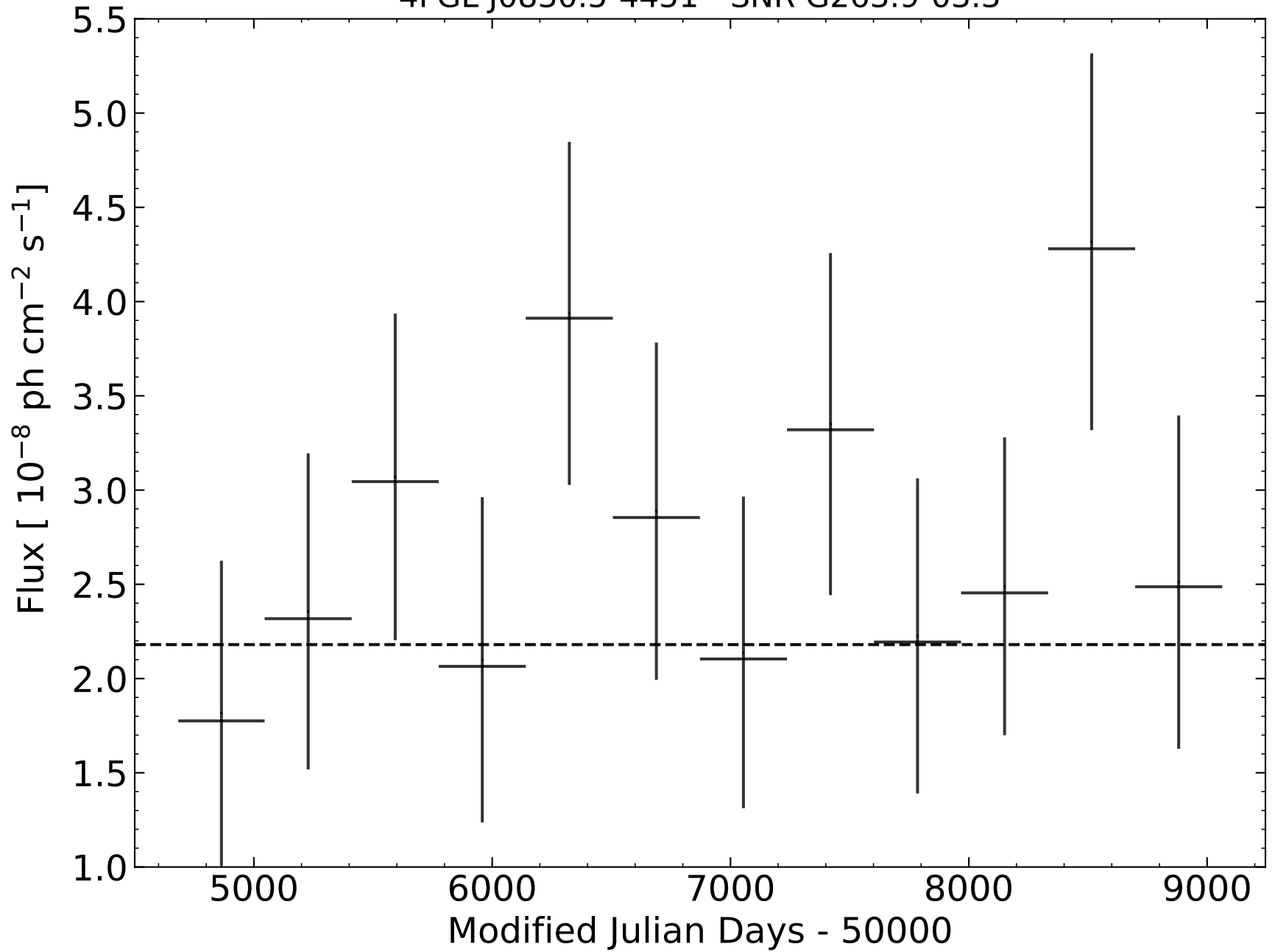
4FGL J0830.5-4451 - SNR G263.9-03.3
