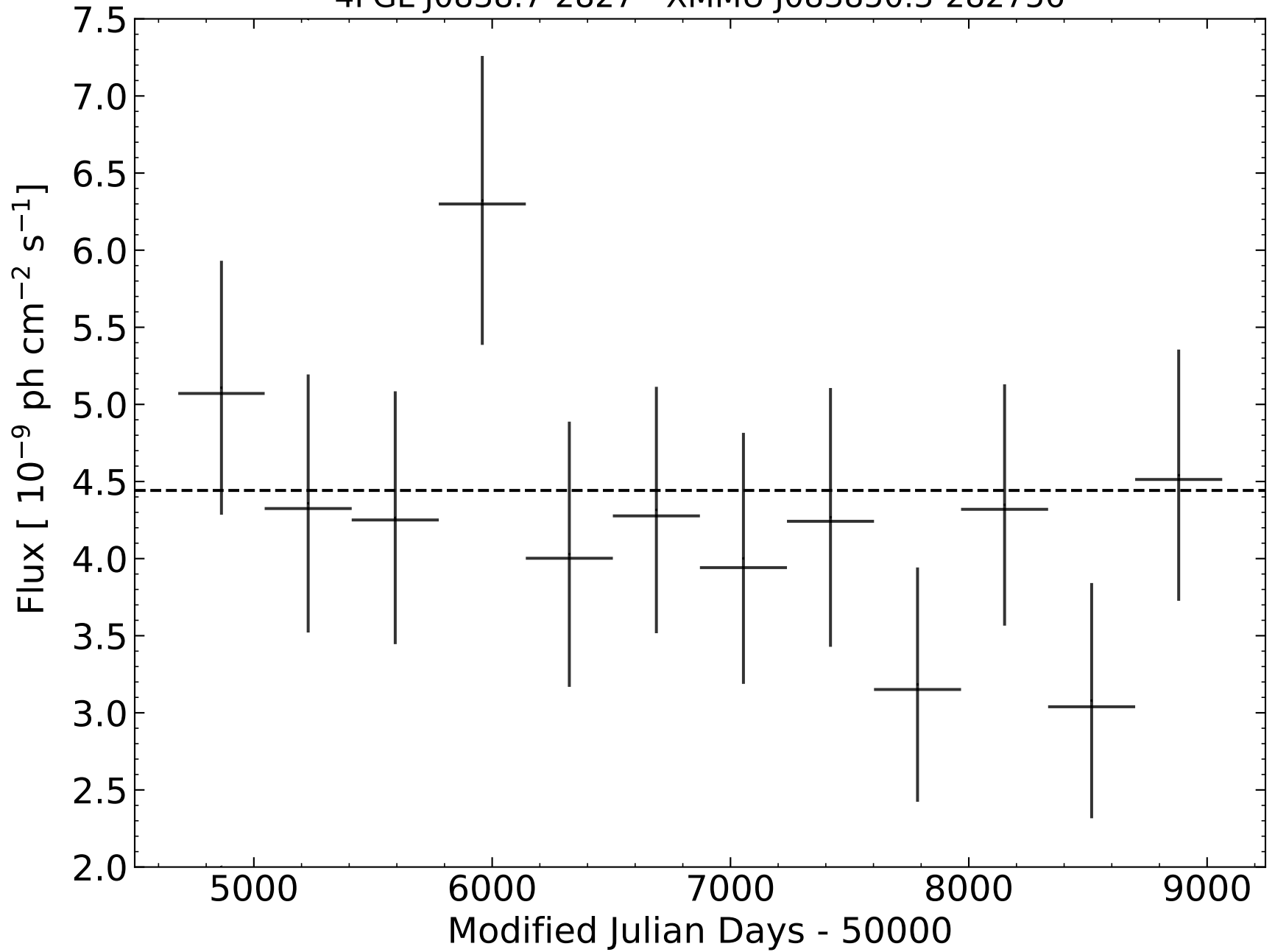
4FGL J0838.7-2827 - XMMU J083850.3-282756
