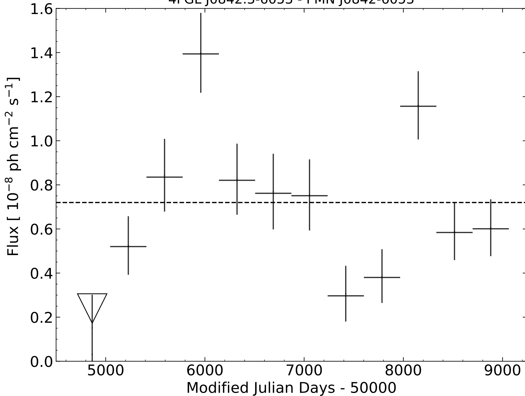
4FGL J0842.3-6053 - PMN J0842-6053
