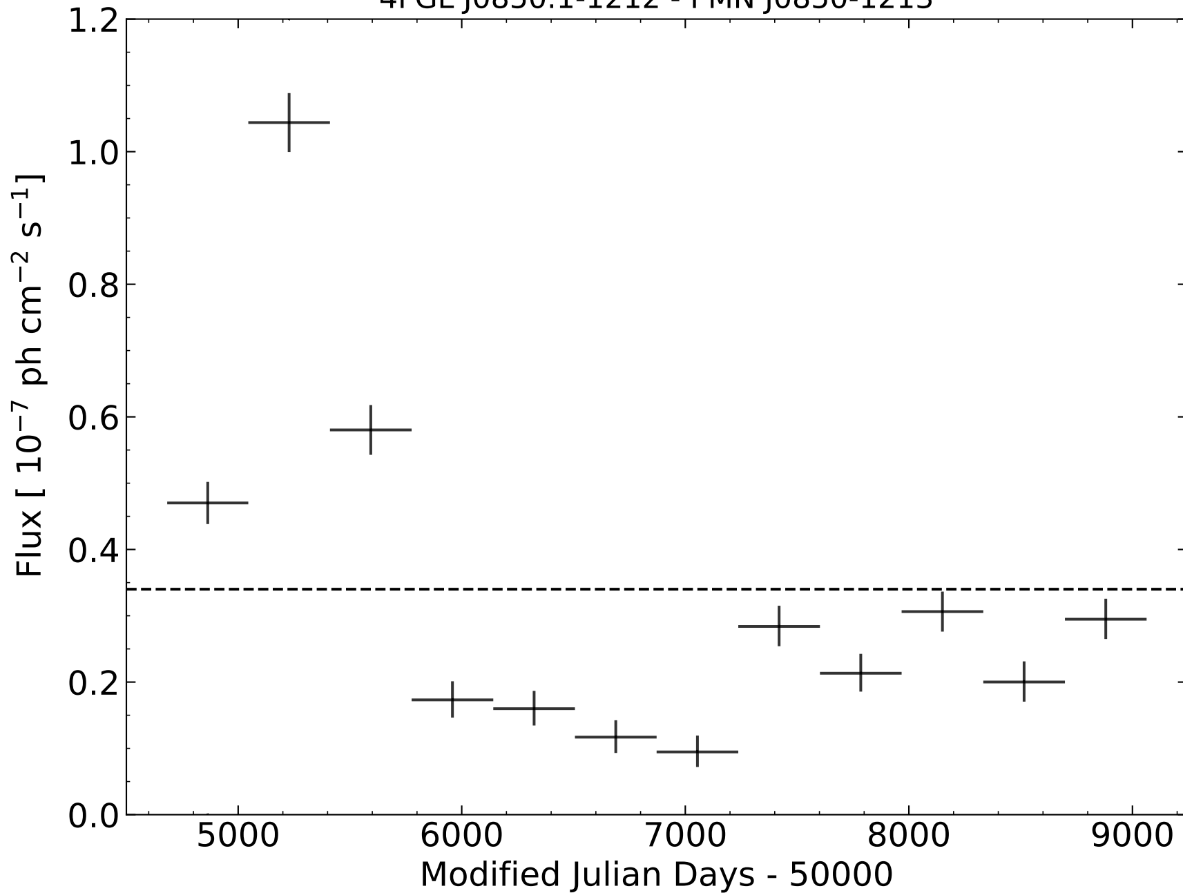
4FGL J0850.1-1212 - PMN J0850-1213
