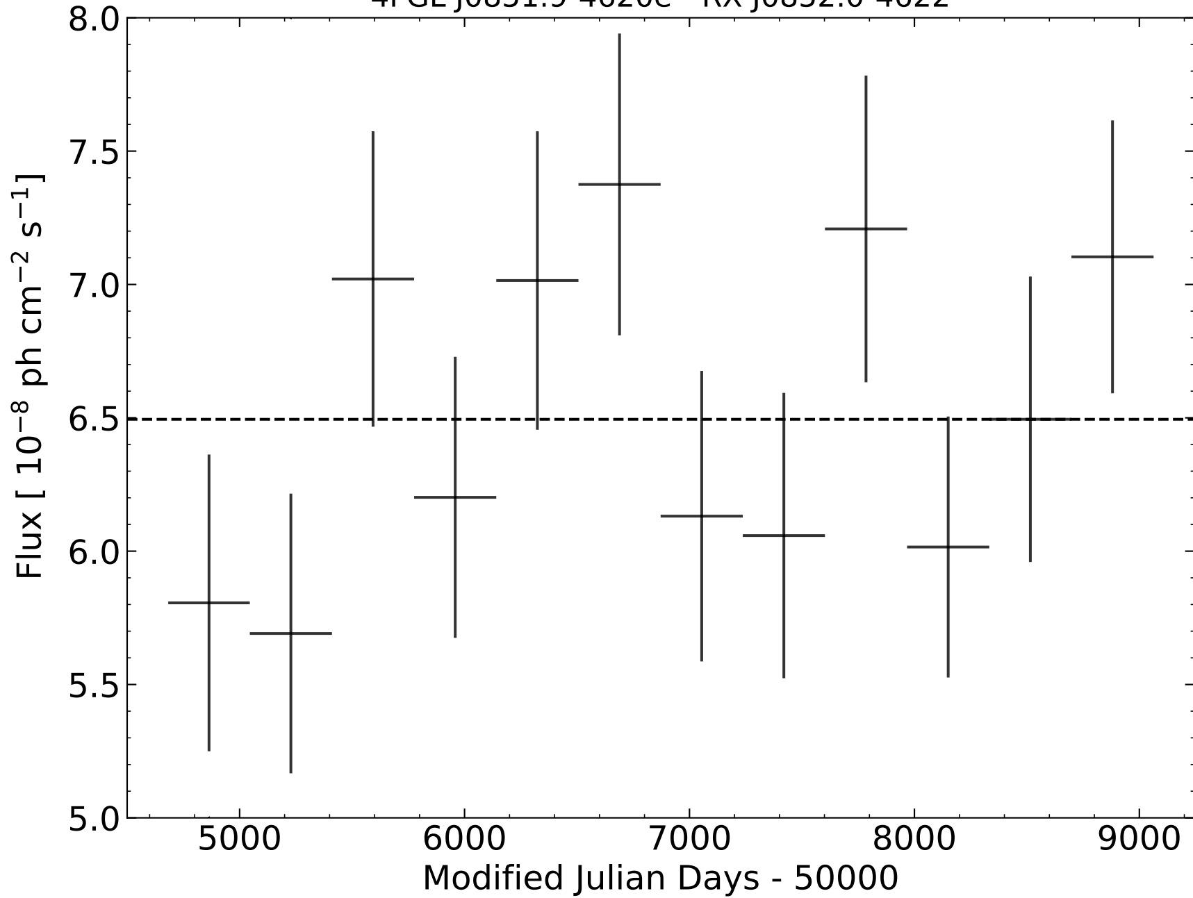
4FGL J0851.9-4620e - RX J0852.0-4622
