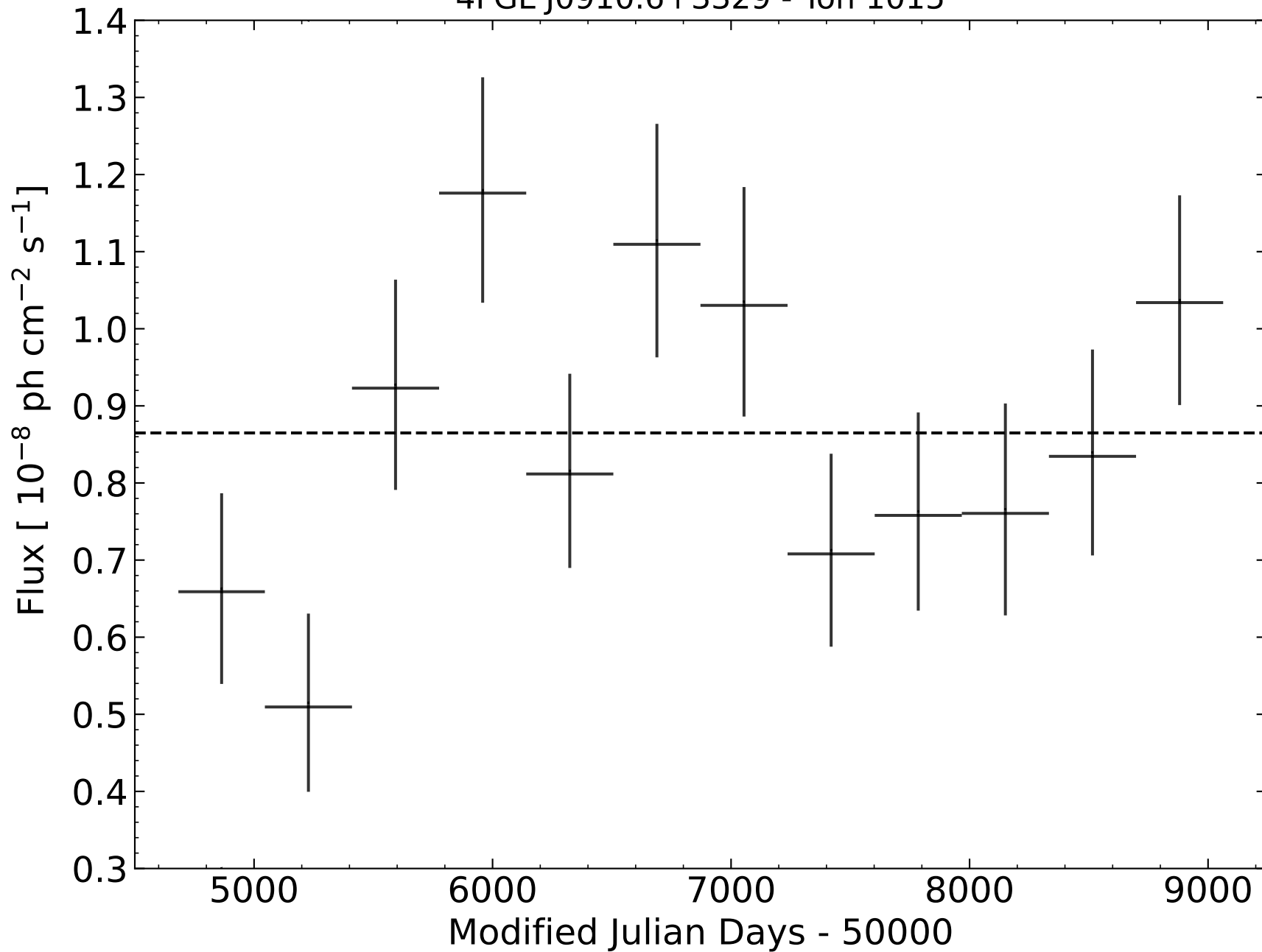
4FGL J0910.6+3329 - Ton 1015
