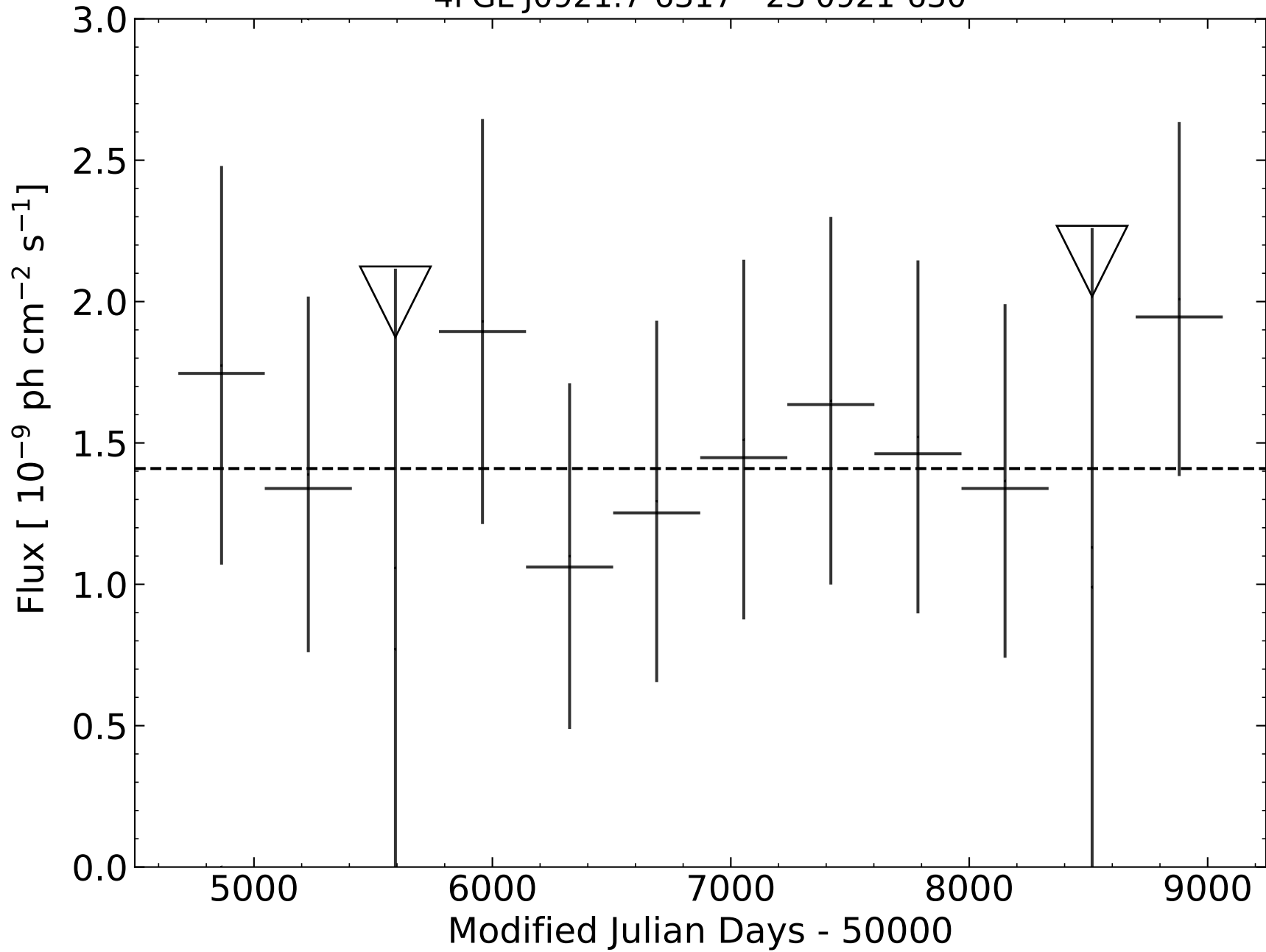
4FGL J0921.7-6317 - 2S 0921-630
