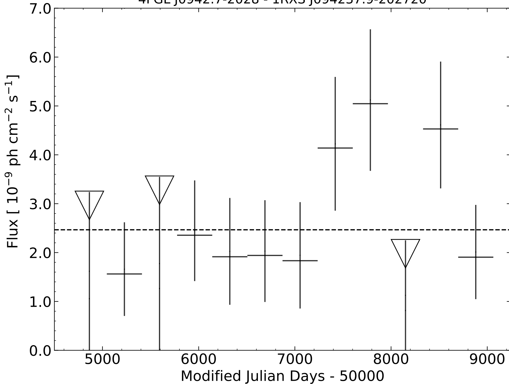
4FGL J0942.7-2028 - 1RXS J094237.9-202720
