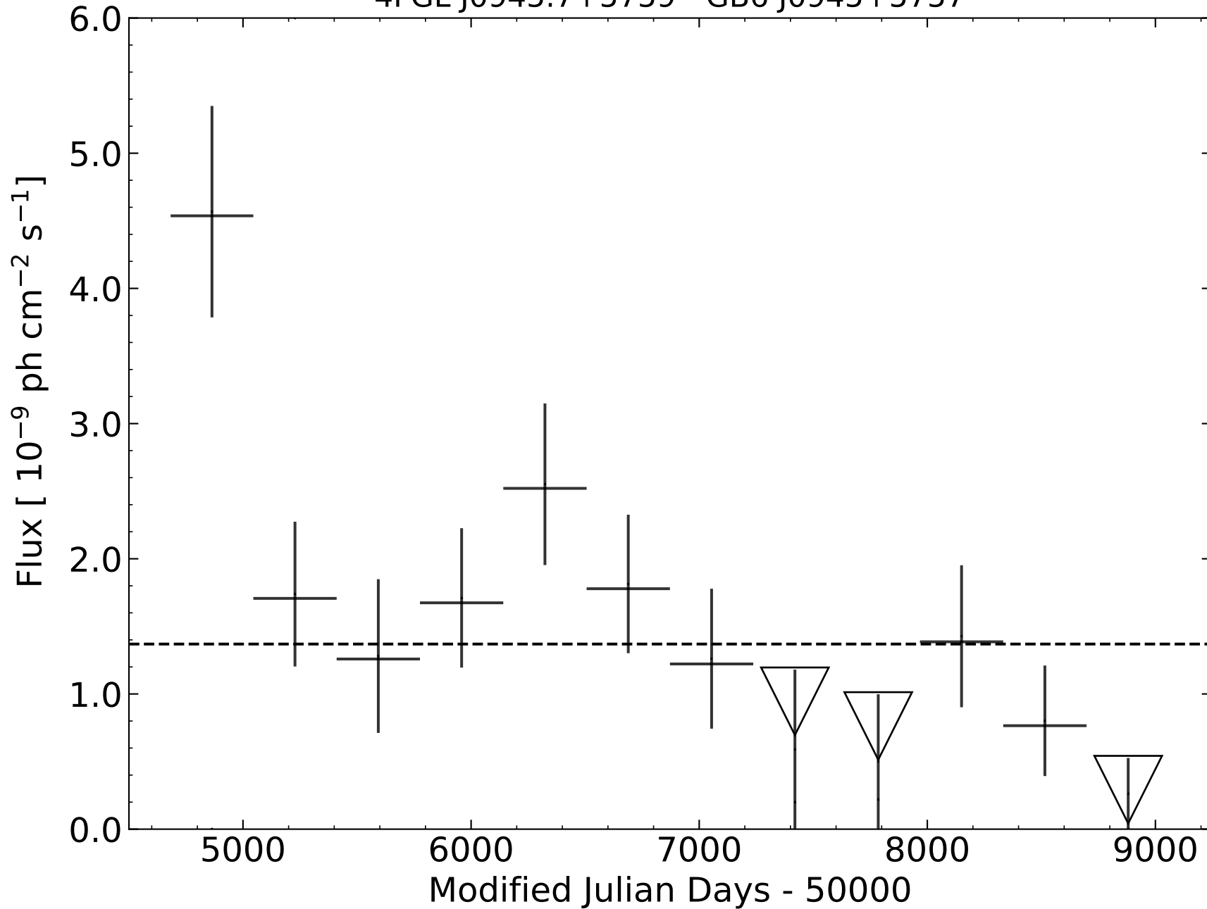
4FGL J0945.7+5759 - GB6 J0945+5757
