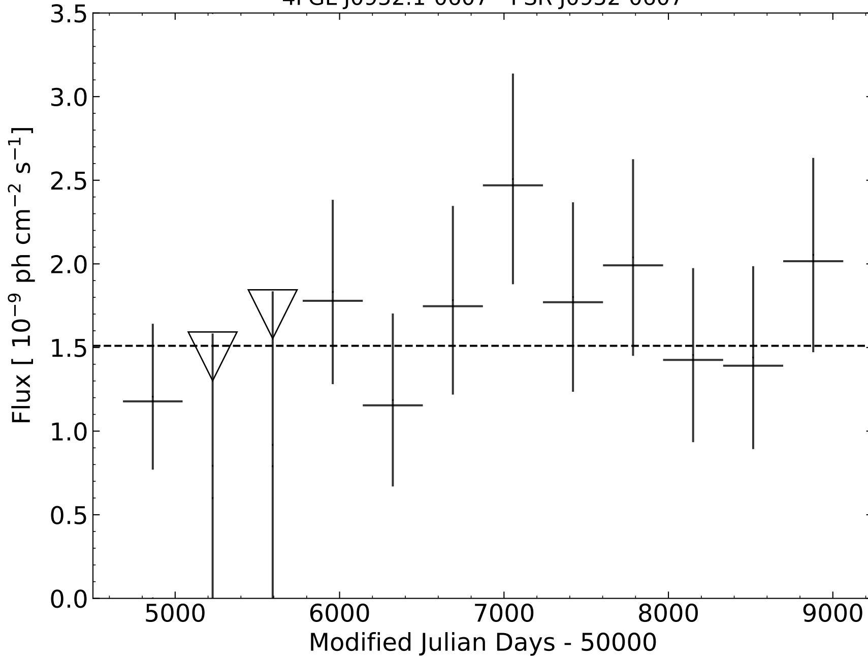
4FGL J0952.1-0607 - PSR J0952-0607
