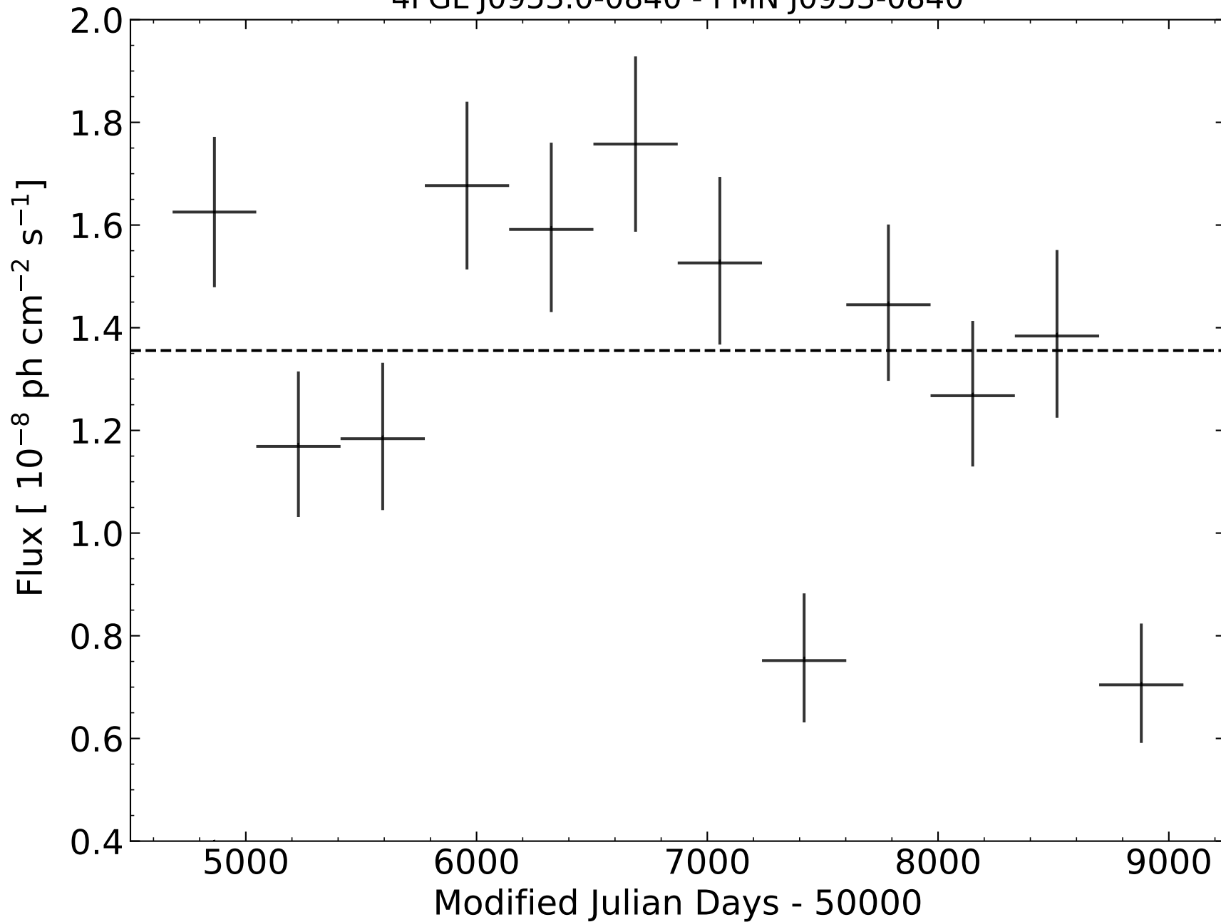
4FGL J0953.0-0840 - PMN J0953-0840
