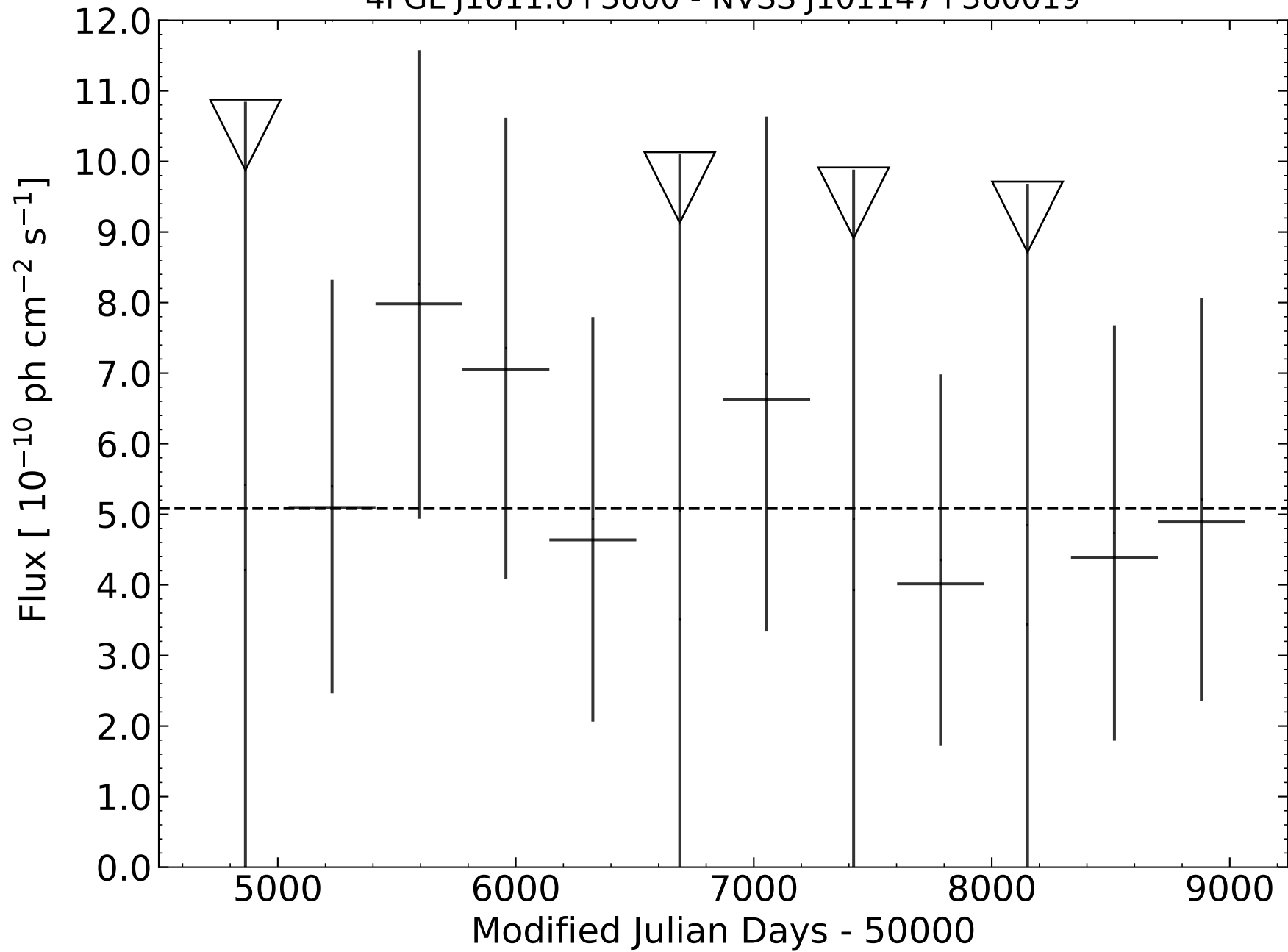
4FGL J1011.6+3600 - NVSS J101147+360019
