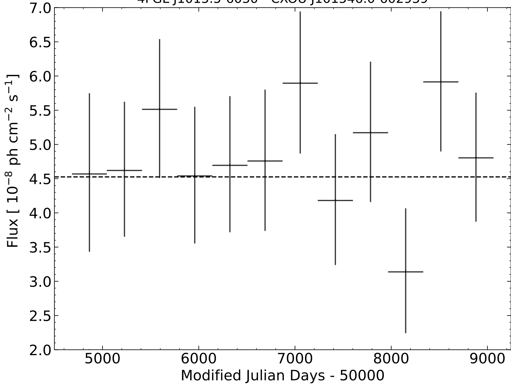
4FGL J1015.5-6030 - CXOU J101546.0-602939
