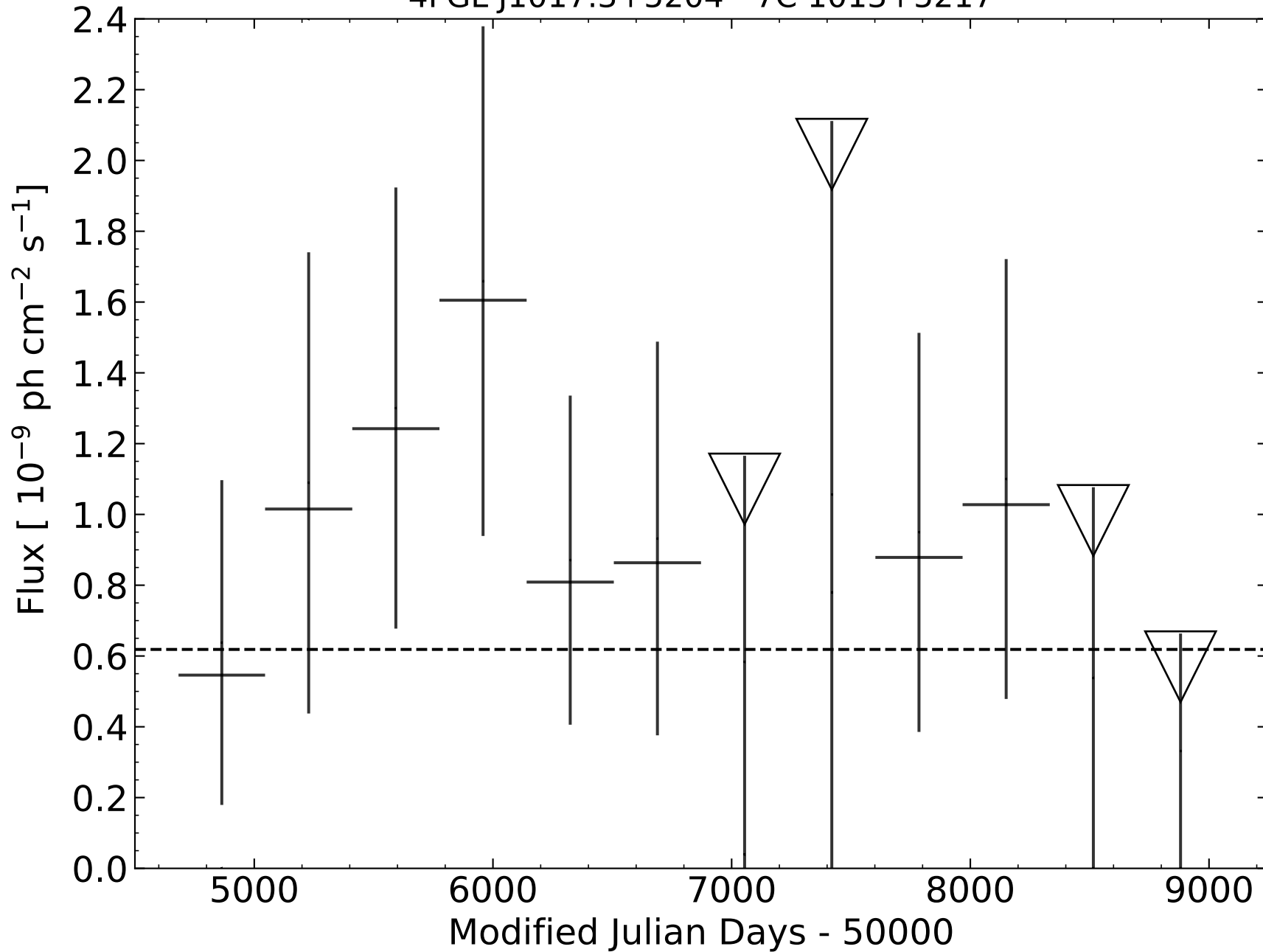
4FGL J1017.3+5204 - 7C 1013+5217
