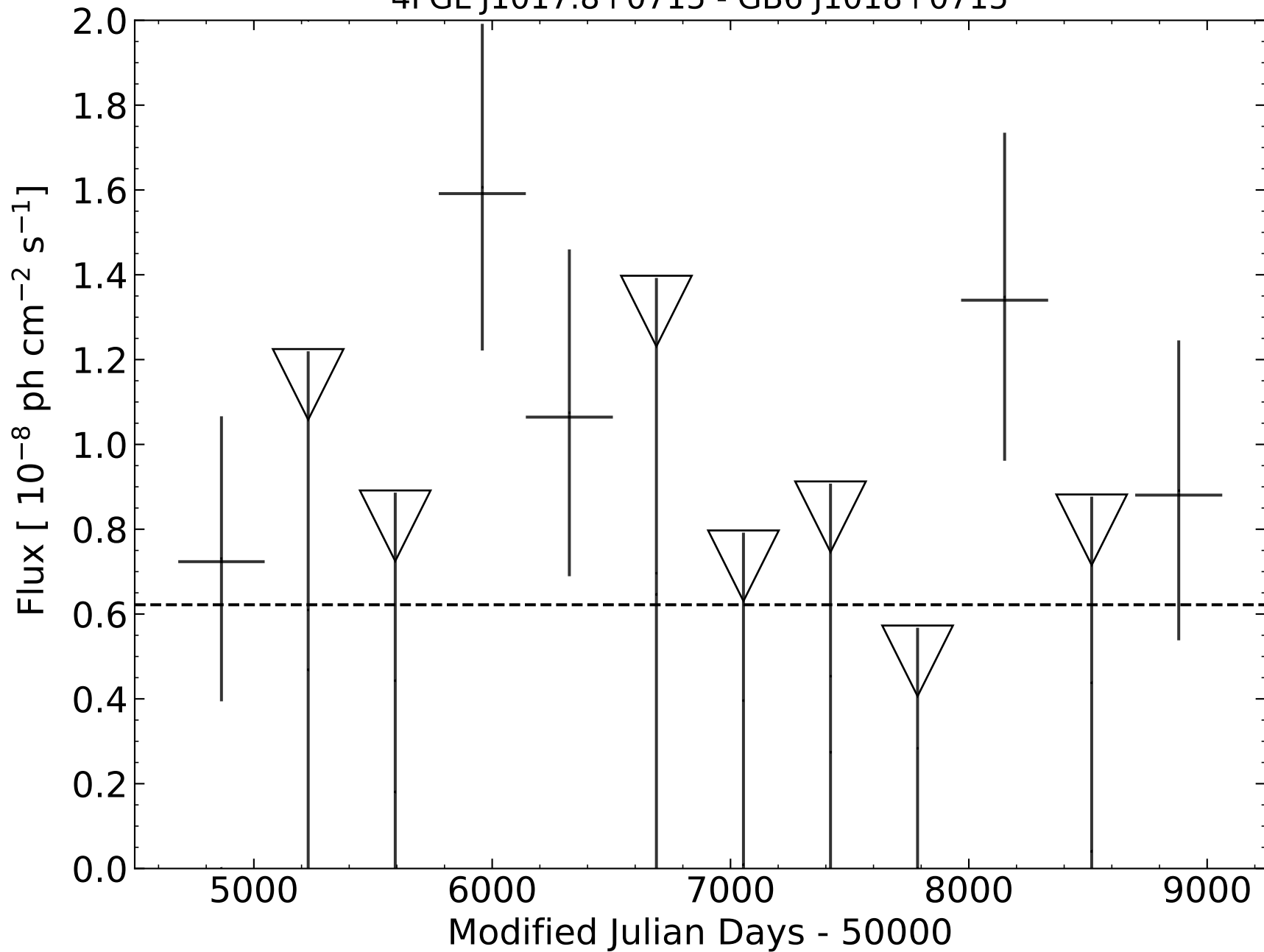
4FGL J1017.8+0715 - GB6 J1018+0715
