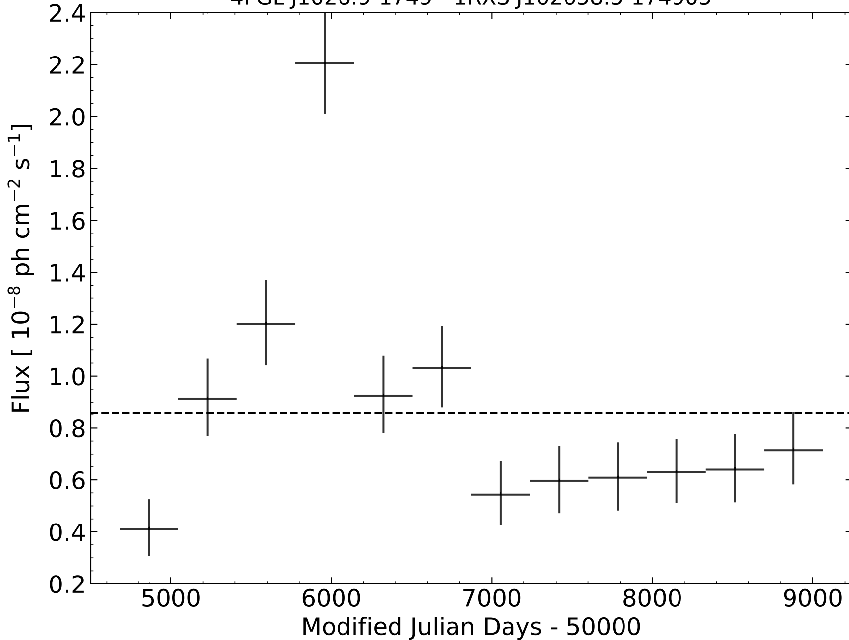
4FGL J1026.9-1749 - 1RXS J102658.5-174905
