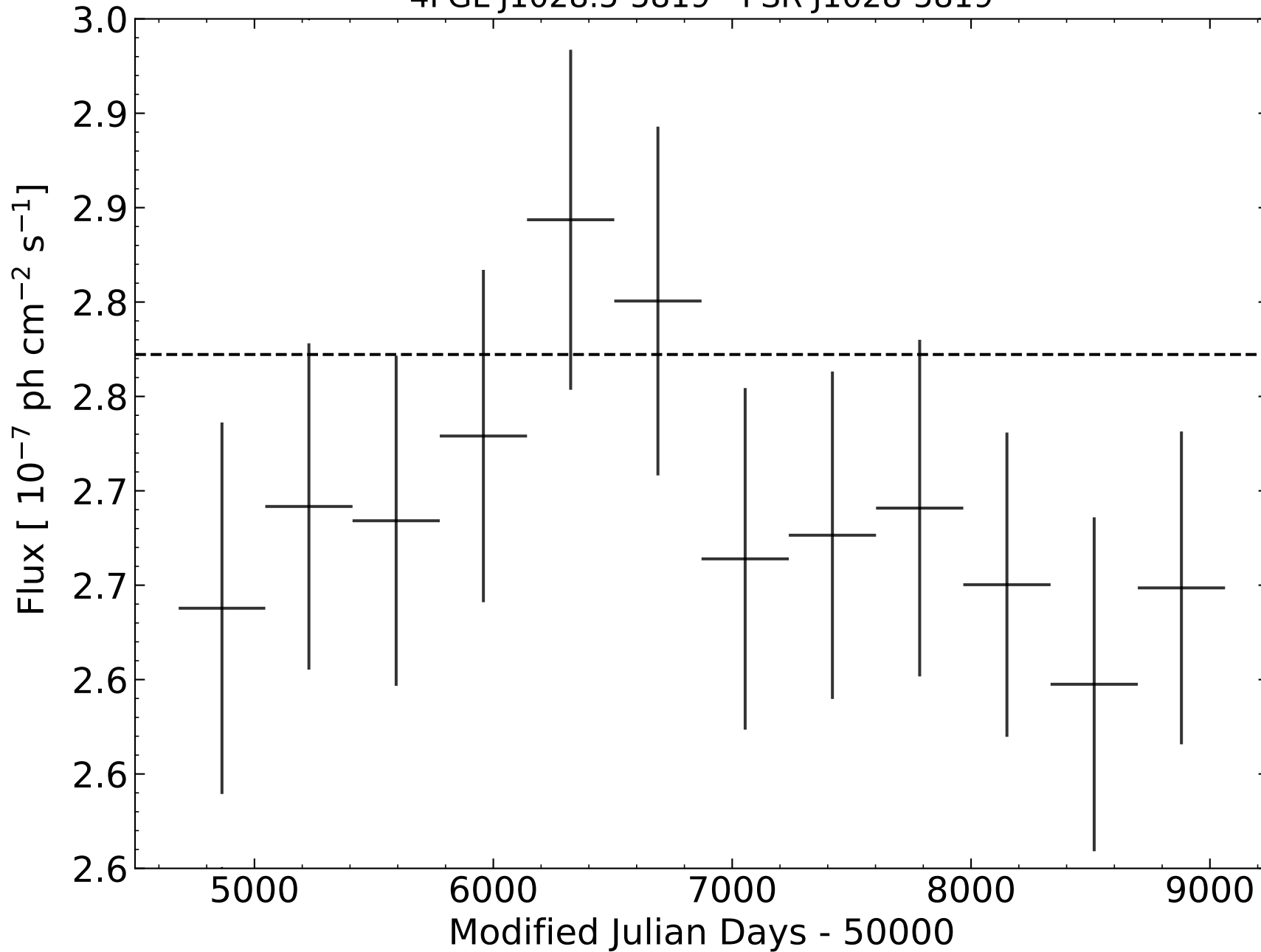
4FGL J1028.5-5819 - PSR J1028-5819
