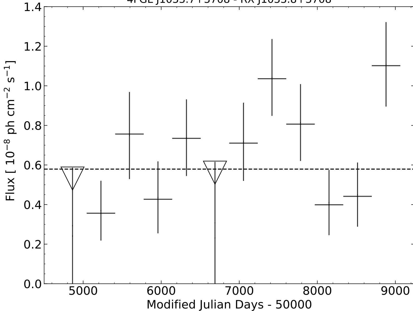
4FGL J1033.7+3708 - RX J1033.8+3708
