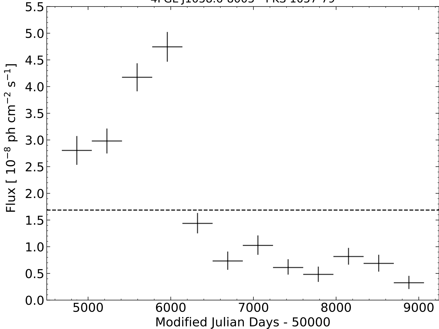
4FGL J1058.6-8003 - PKS 1057-79
