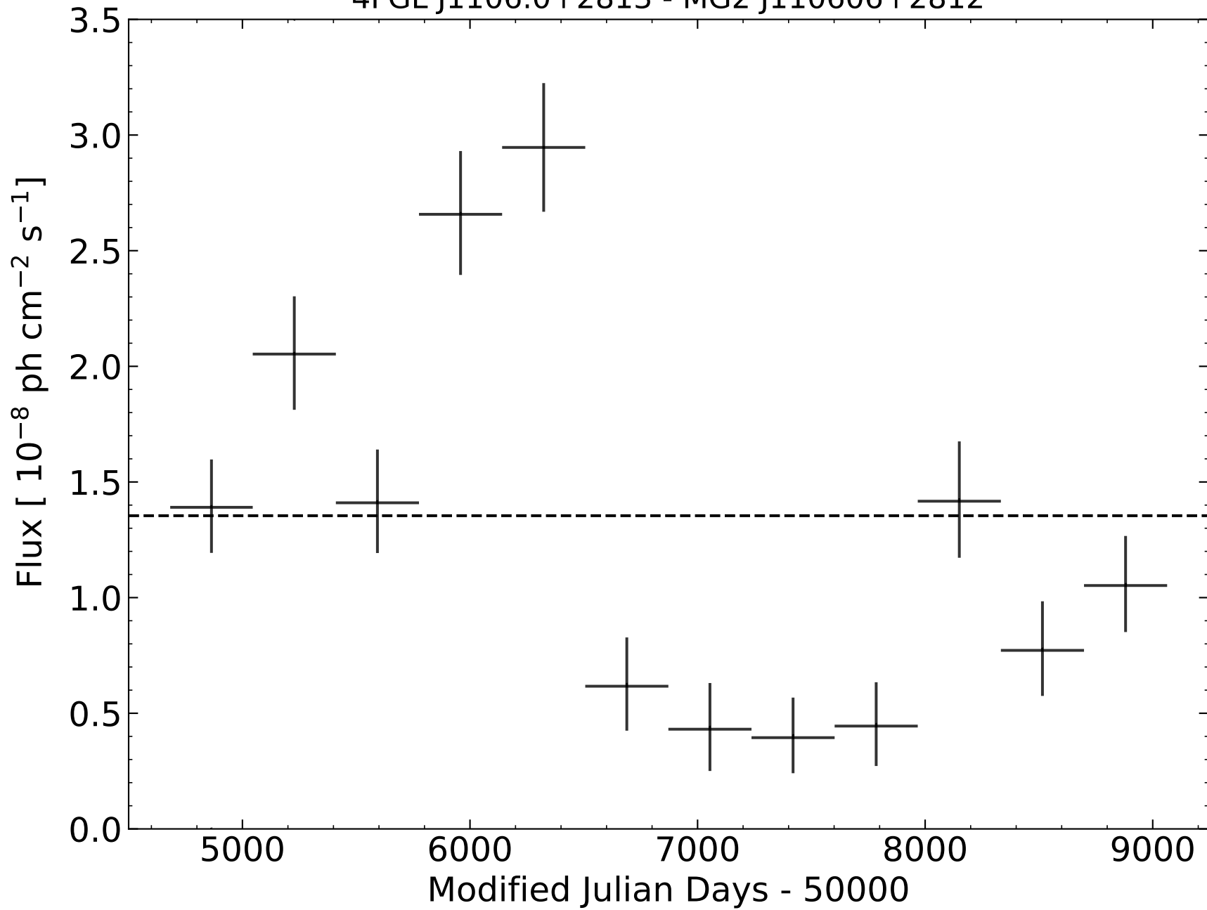
4FGL J1106.0+2813 - MG2 J110606+2812
