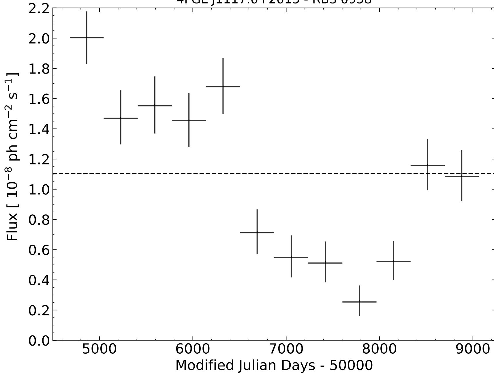
4FGL J1117.0+2013 - RBS 0958
