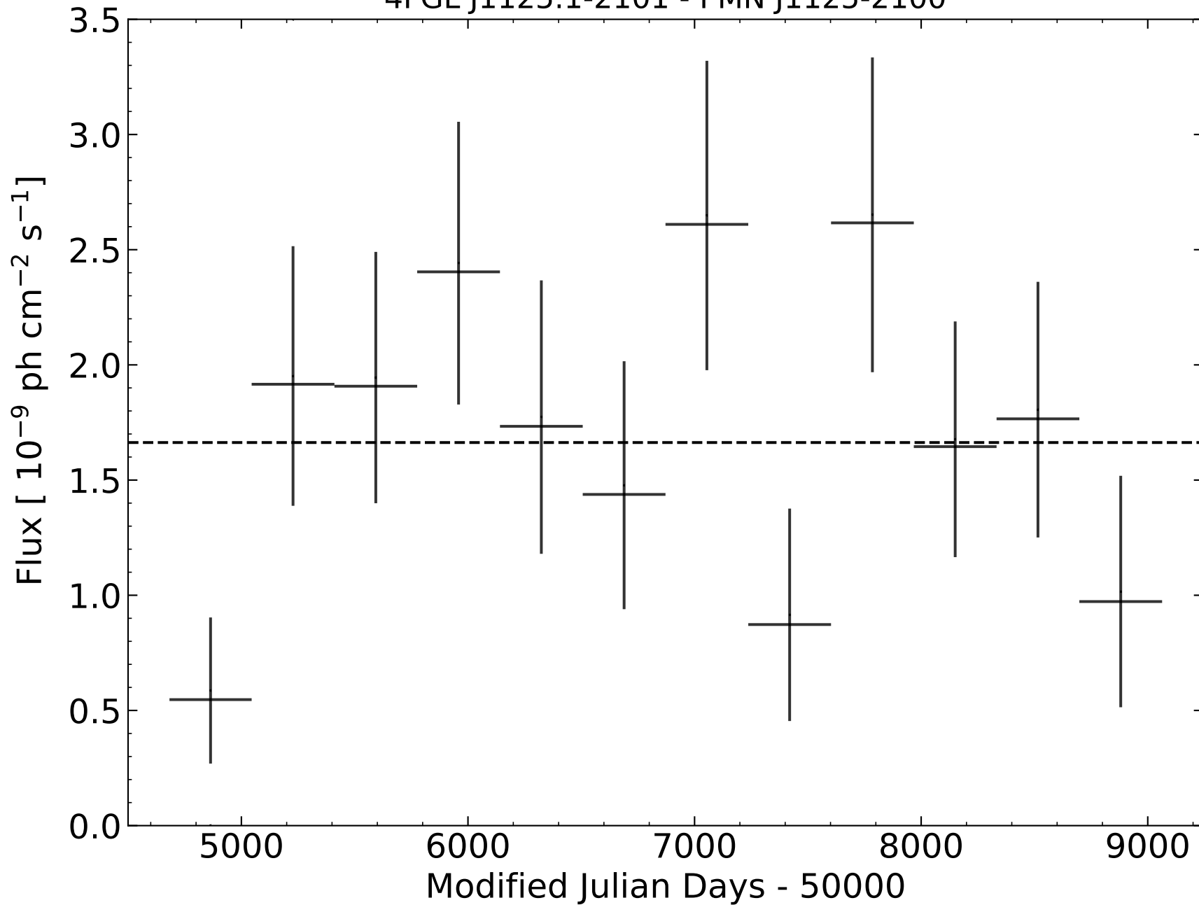
4FGL J1125.1-2101 - PMN J1125-2100
