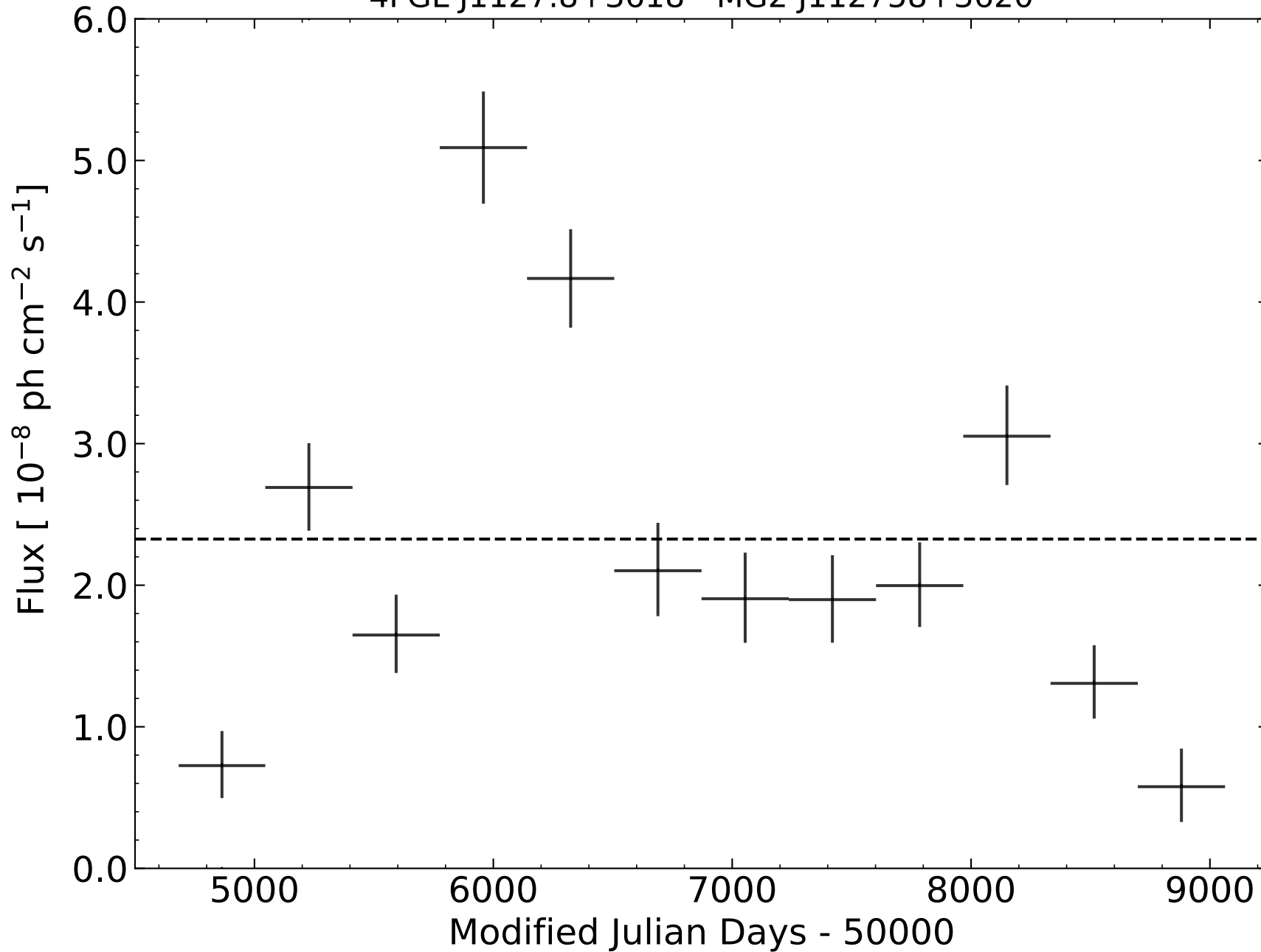
4FGL J1127.8+3618 - MG2 J112758+3620
