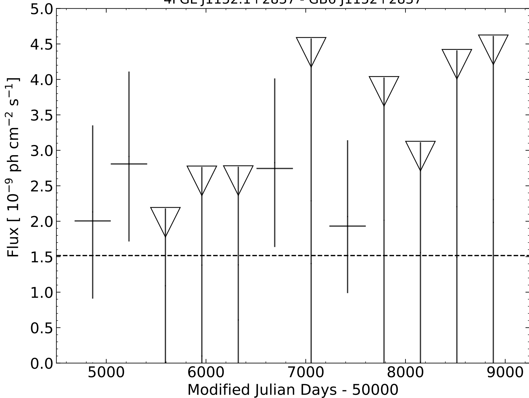
4FGL J1152.1+2837 - GB6 J1152+2837
