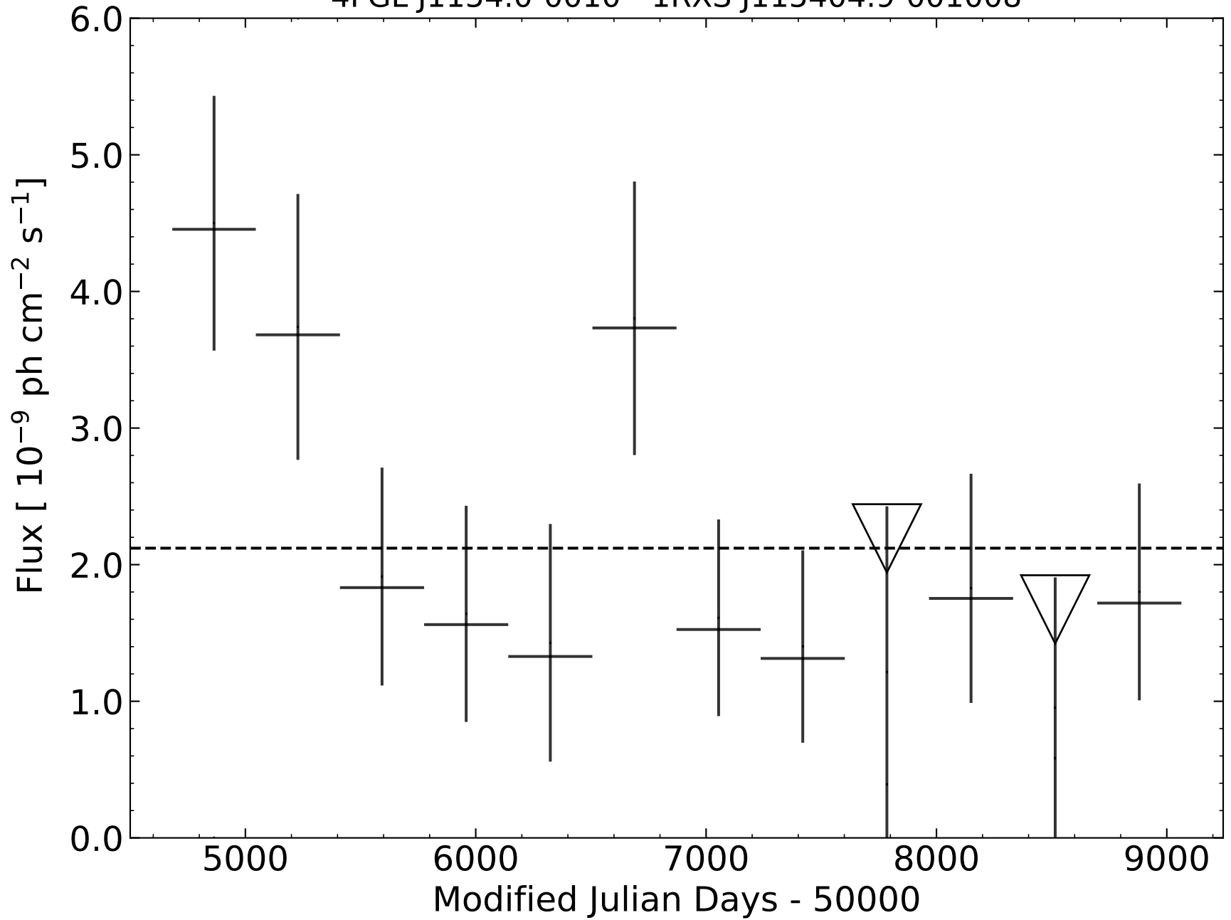
4FGL J1154.0-0010 - 1RXS J115404.9-001008
