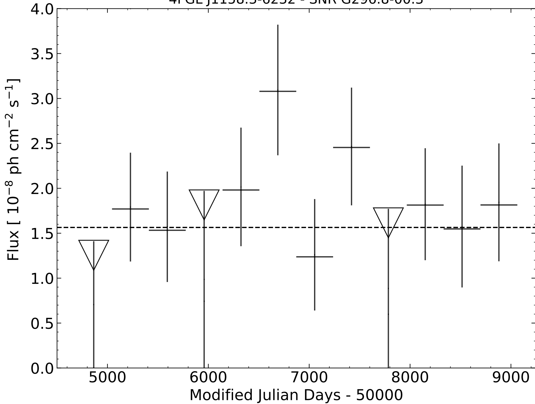
4FGL J1158.3-6232 - SNR G296.8-00.3
