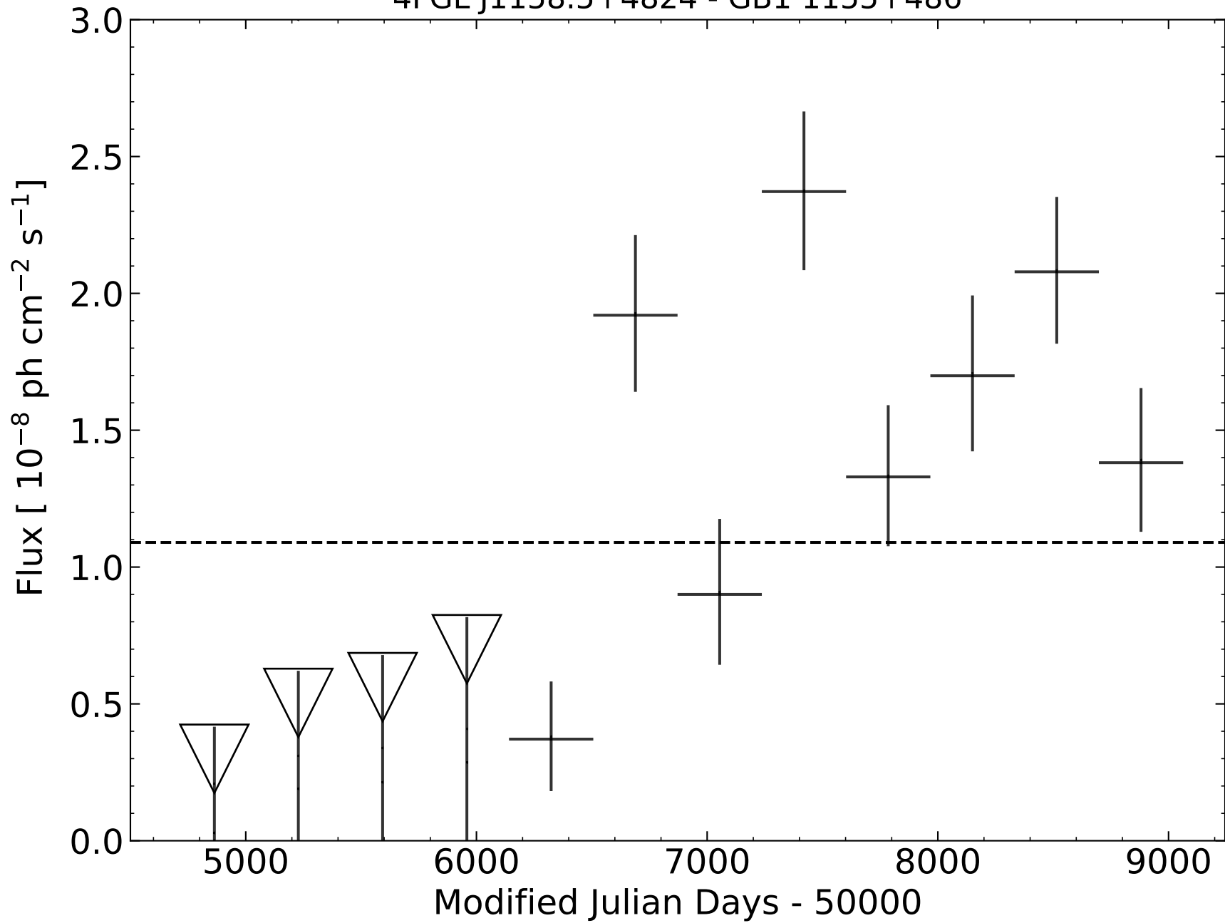
4FGL J1158.5+4824 - GB1 1155+486
