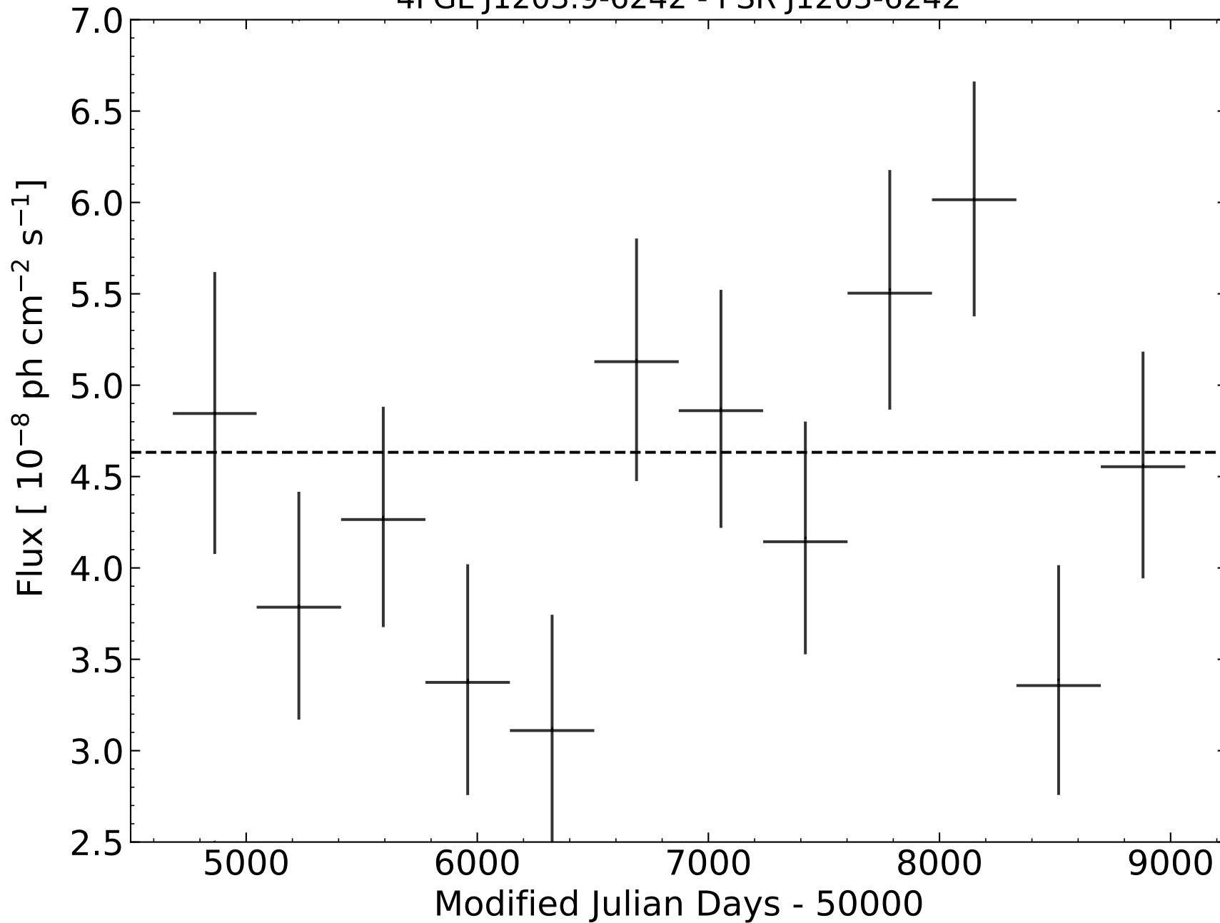
4FGL J1203.9-6242 - PSR J1203-6242
