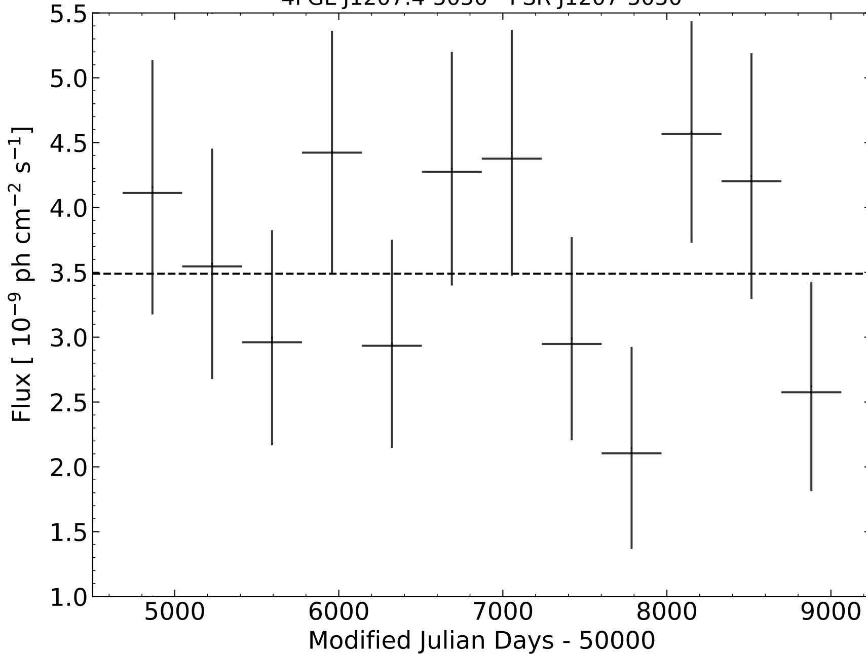
4FGL J1207.4-5050 - PSR J1207-5050
