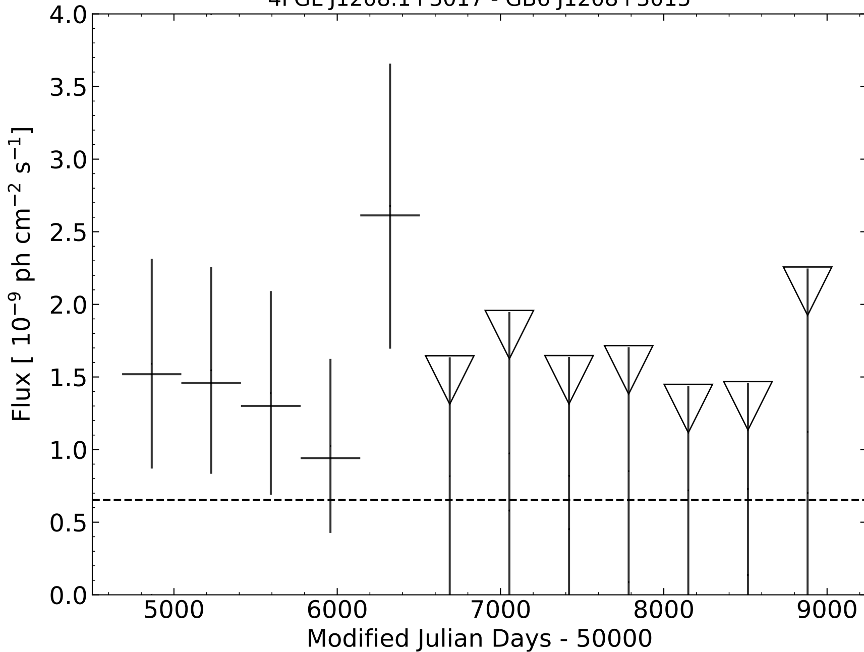
4FGL J1208.1+3017 - GB6 J1208+3015
