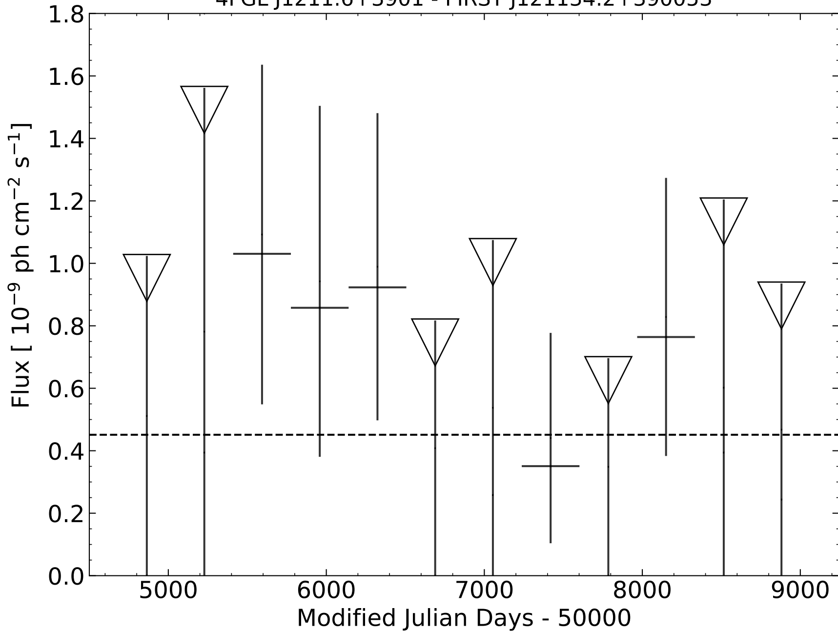
4FGL J1211.6+3901 - FIRST J121134.2+390053
