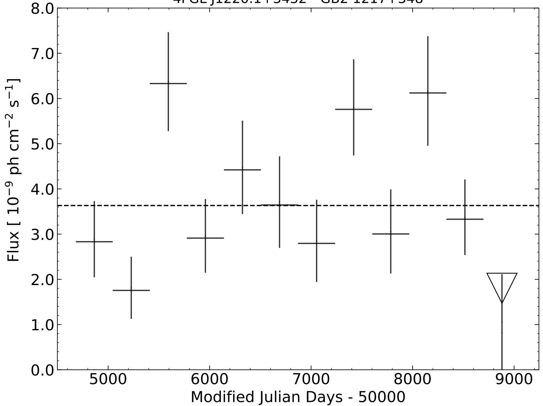
4FGL J1220.1+3432 - GB2 1217+348
