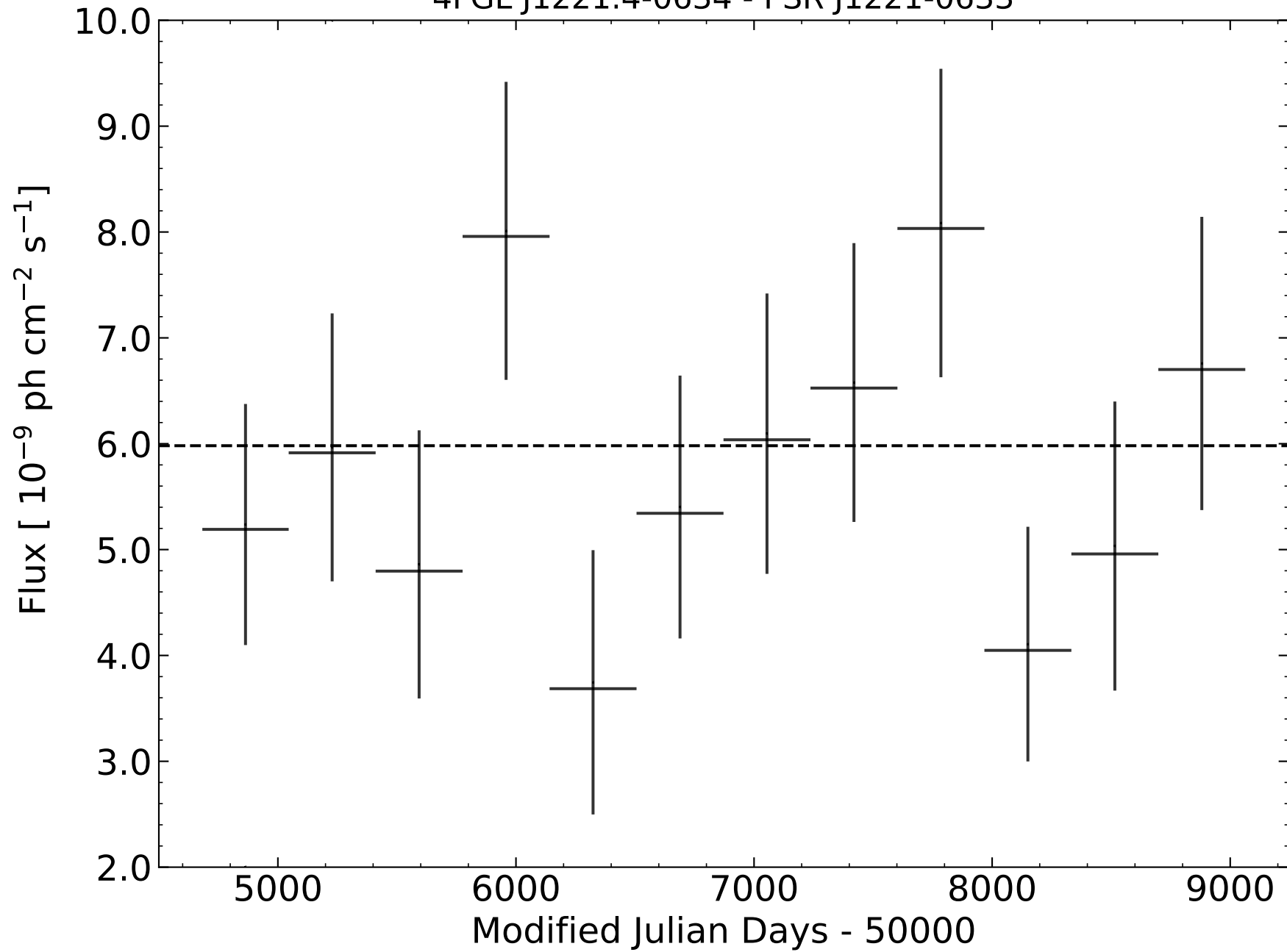
4FGL J1221.4-0634 - PSR J1221-0633
