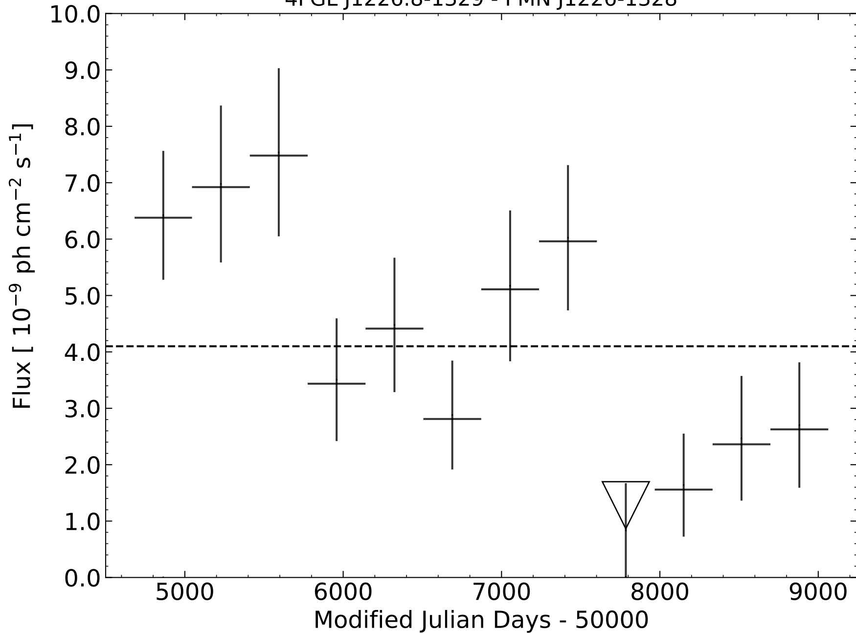
4FGL J1226.8-1329 - PMN J1226-1328
